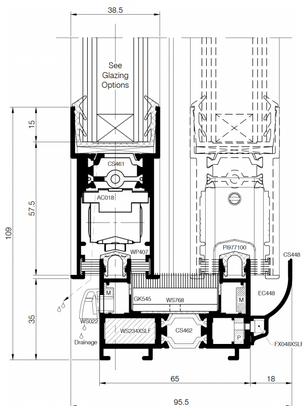
Sill Details Standard Frame
