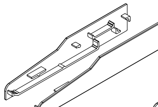
EC894 155mm SILL END CAP
