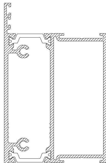
CS866 ECO DOOR TRANSOM (OPEN IN)
