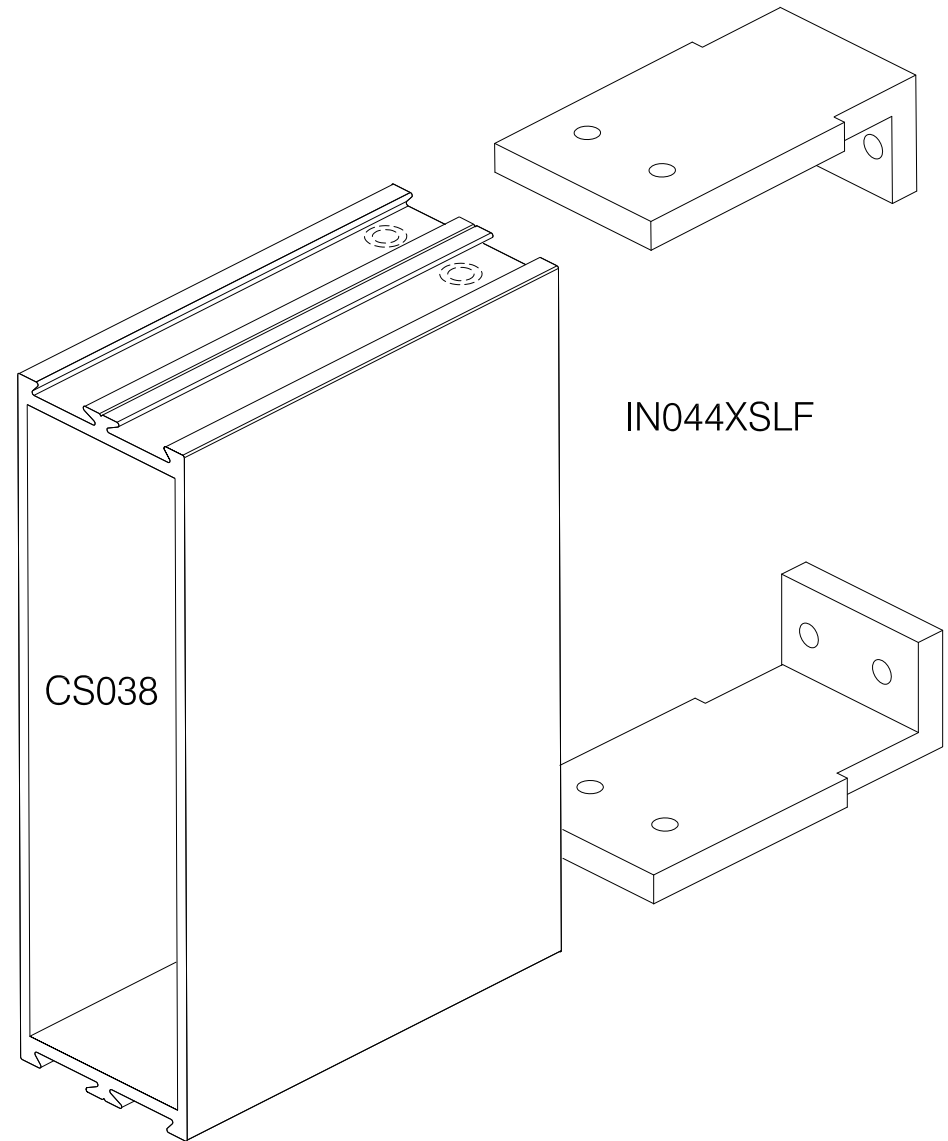
RAIL FIXING CLEAT PRE-DRILLED FOR M5 FIXINGS (FX079XSLF)
