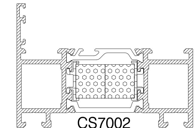
CS7002 55mm FLAT FACE FOLDING DOOR LEAF
