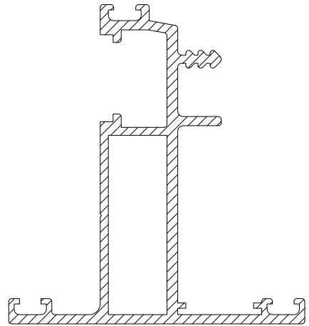
AT201 VENT FRAME ALUMINIUM
