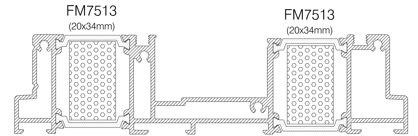
CS7500 DOUBLE TRACK HEAD & THRESHOLD
