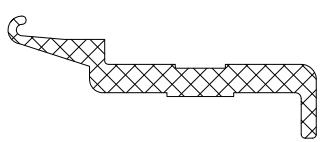
GK546 OVERLAP STILE INTERLOCK INSERT
