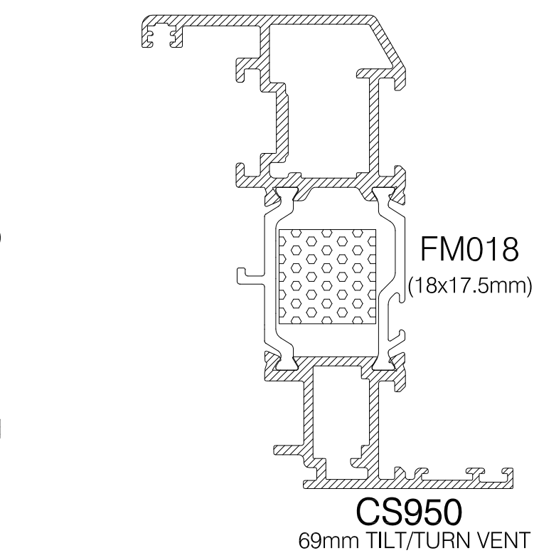
CS950 69mm TILT/TURN VENT
