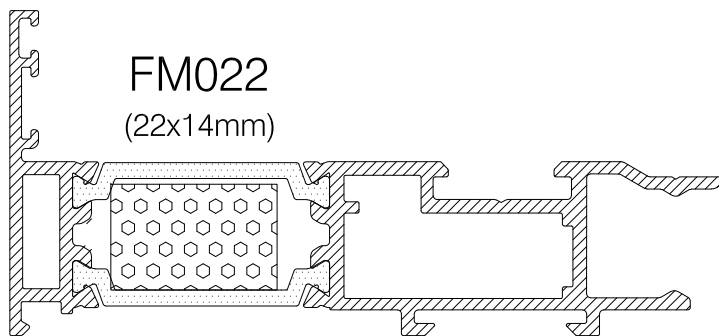
CS7511 TRIPLE TRACK OUTERFRAME
