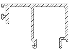
CS926 GLAZING BEAD 17-23mm
