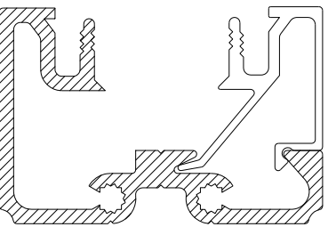
CS028 FIXED BEAD CARRIER
