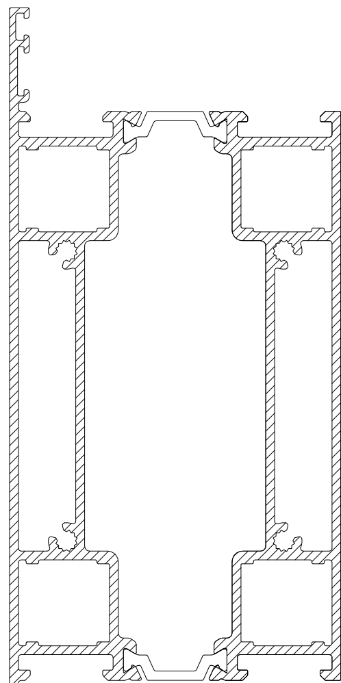
CS781 150mm TRANSOM/MIDRAIL
