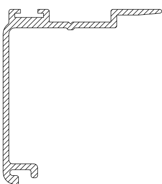
CS452 OVERLAP STILE INTERLOCK
