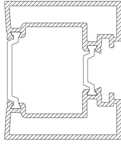
CS998 MULLION DOOR ADAPTOR
