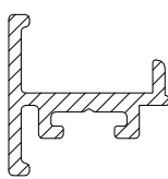
CS883 LOW THRESHOLD GASKET CARRIER OPEN OUT
