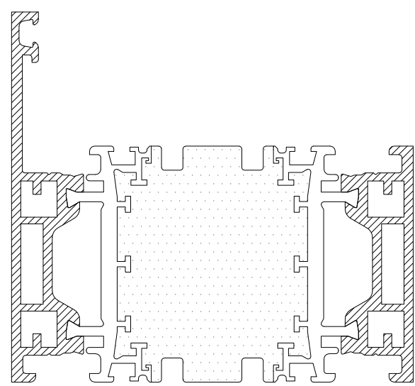
10-701 75mm OUTER FRAME / FIXED LIGHT
