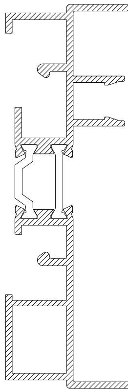
CS465 2 TRACK DOOR INSIDE TRACK JAMB
