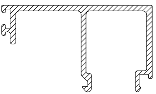
CS924 GLAZING BEAD 7-11mm
