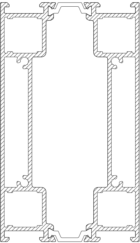
CS783 110mm SECURITY OPTION DOOR MIDRAIL
