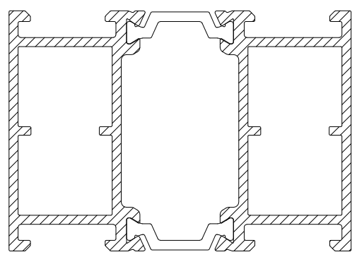
CS799 45mm TRANSOM / MIDRAIL
