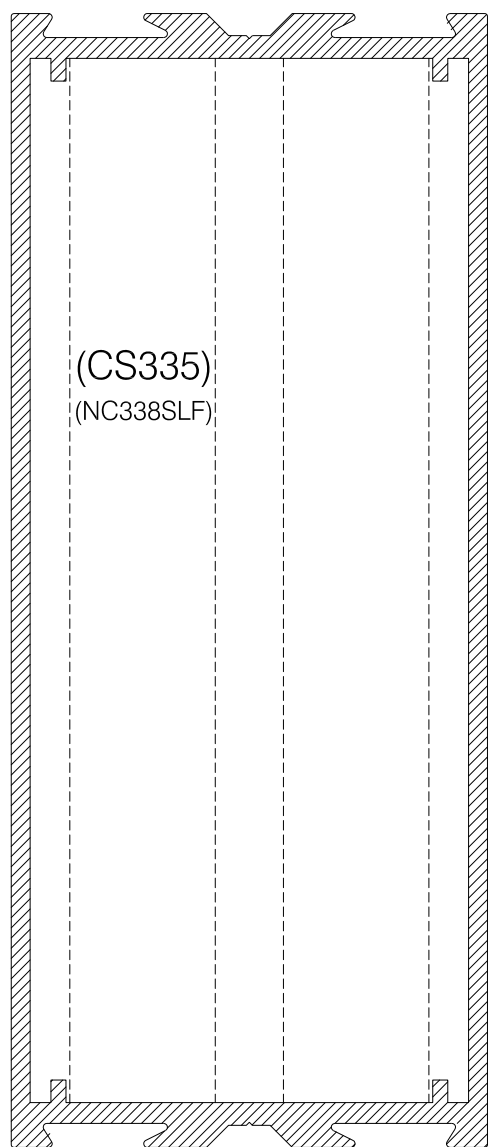
CS338 150mm DOUBLE GLAZED SASH / TRANSOM (63mmW)
