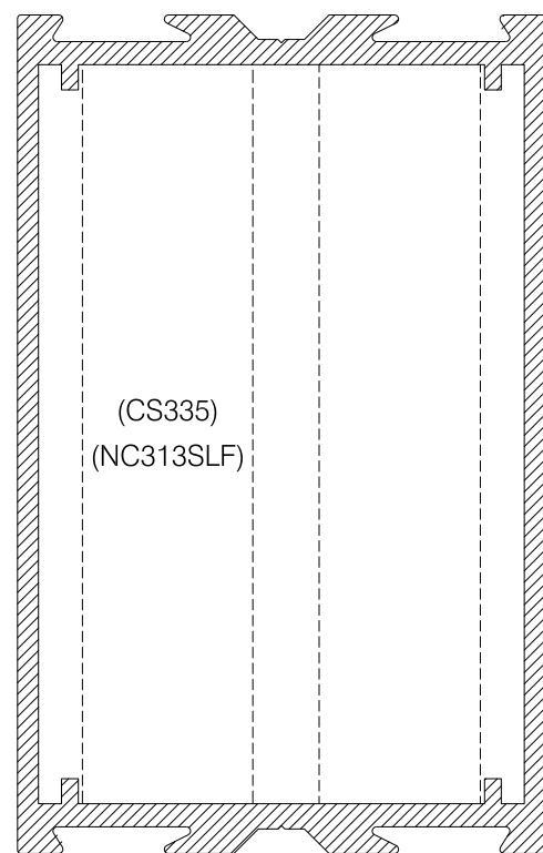
CS313 100mm DOUBLE GLAZED SASH / TRANSOM (63mmW)
