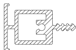
AT202 FRAME NOSE ALUMINIUM
