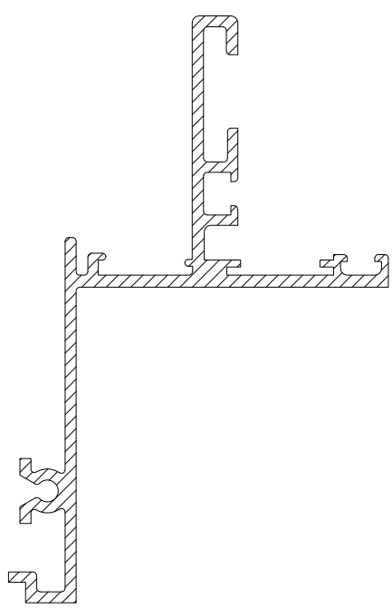
AT212 OUTERFRAME ADAPTOR ALUMINIUM
