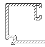
CS823 GLAZING BEAD FOR 28 MM GLASS
