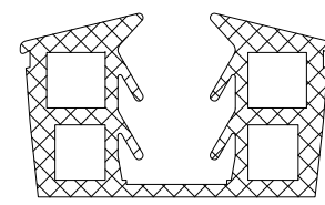
GK410 10 - 12mm GLASS GLAZING GASKET
