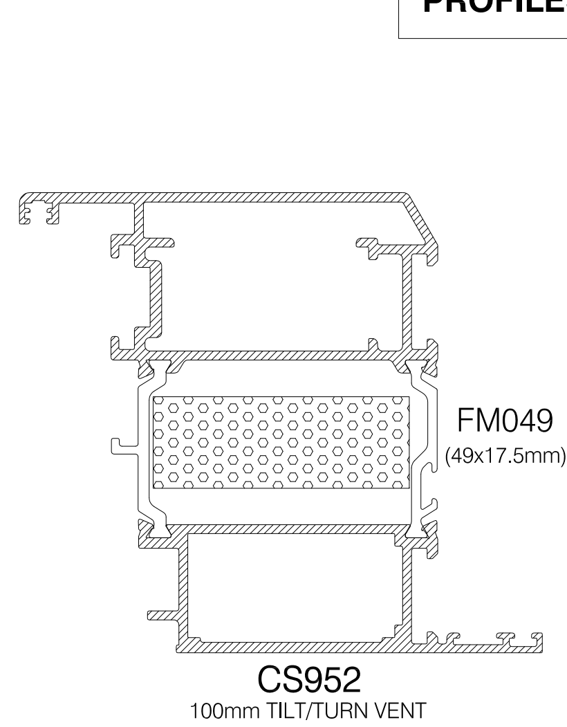
CS952 100mm TILT/TURN VENT
