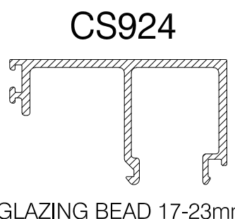
GLAZING BEAD 17-23mm
