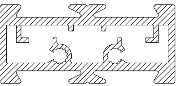
CS115 20mm TRANSOM MULLION
