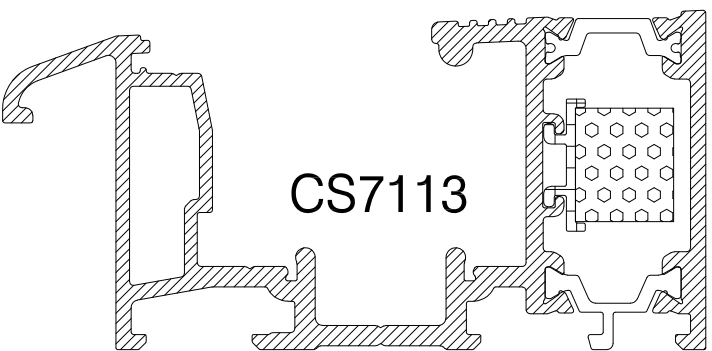
SINGLE RAMP SILL TRACK
