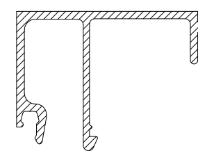
10-963 GLAZING BEAD 36mm
