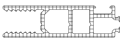
6782 48mm END CLOSURE
