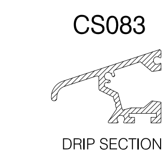
CS083 DRIP SECTION
