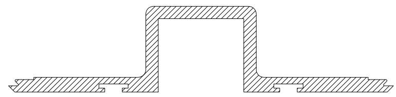
CS042 SLIDING FOLDING DOOR'S HEADER BAR
