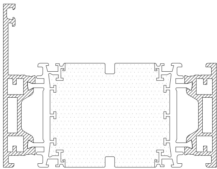
10-901 90mm OUTER FRAME / FIXED LIGHT
