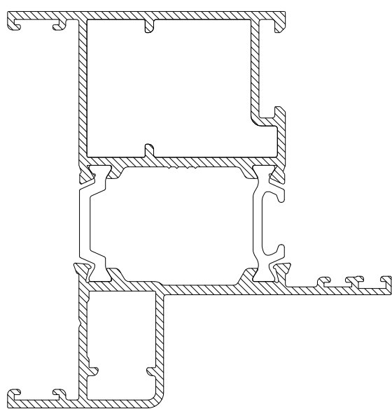
CS862 75mm DOOR OUTER FRAME
