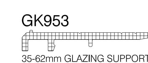
GK953 35-62mm GLAZING SUPPORT
