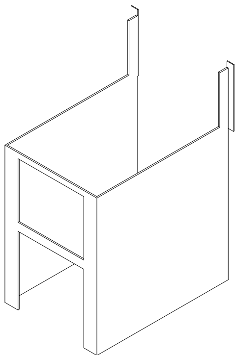
EC461 END CAP FOR CS461(Plastic)
