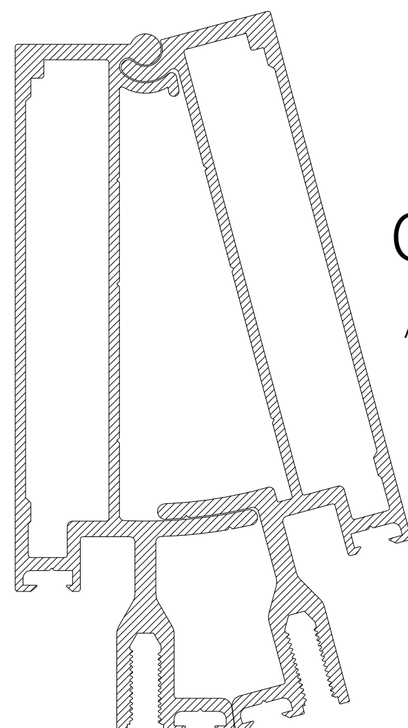
CS610 104mm ADJUSTABLE CORNER MULLION (PART A)
