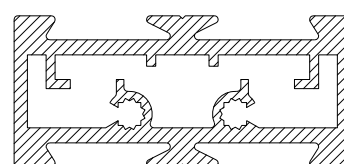
CS115 20mm TRANSOM MULLION
