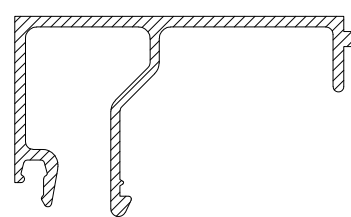
10-965 GLAZING BEAD 45mm
