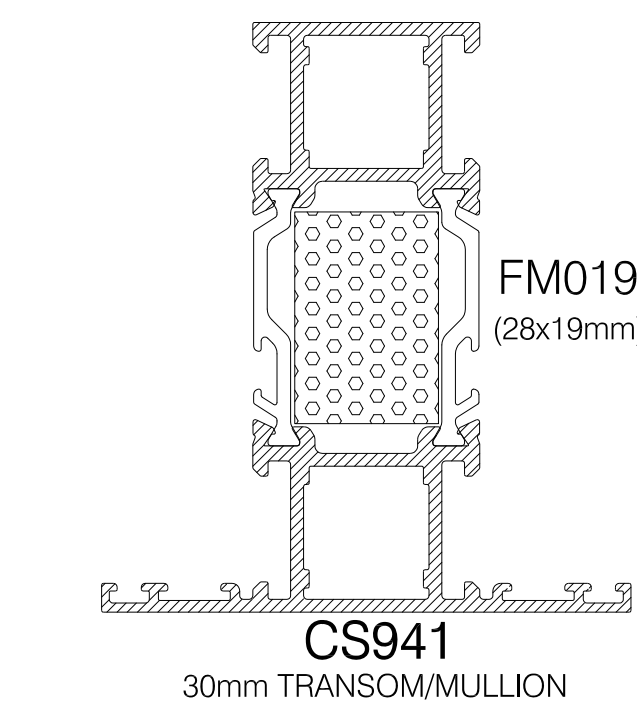
CS941 30mm TRANSOM/MULLION
