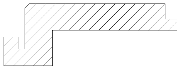
AT321 DOOR VENT TIMBER OPEN OUT
