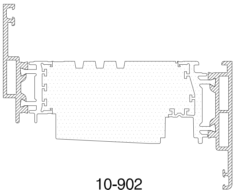
10-902 90mm VENT FRAME
