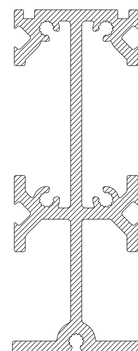
CS659 CURTAIN WALL 90mm SPIGOT
