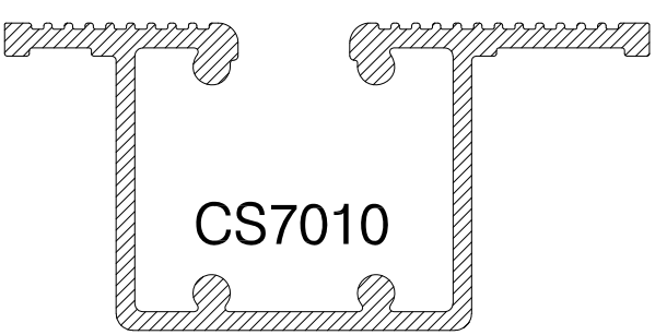
SILL TRACK NON THERMAL SPECIAL ORDER
