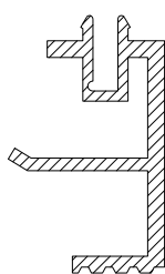
CS633 27mm POCKET FILLER FOR PVC PRESSURE PLATE
