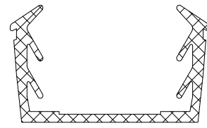
GK428 27 - 29mm GLASS GLAZING GASKET
