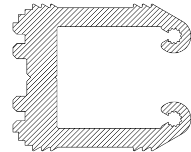
CS035 DOOR SASH WELDING SCREW OR TIE-ROD CLEAT
