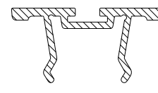
CS084 ARMOURED GLASS POCKET FILLER WOOLPILE CARRIER
