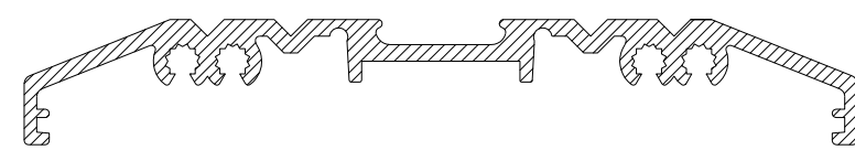
CS315 DOUBLE RAMP DRAINED THRESHOLD
