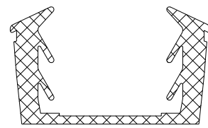
GK424 23 - 25mm GLASS GLAZING GASKET
