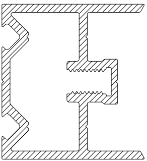
CS791 ADJUSTABLE FINGER GUARD FIXING CHANNEL
