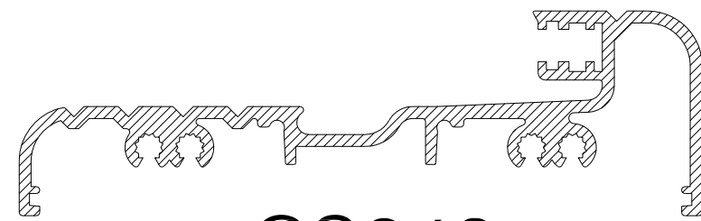
CS348 CENTRE HUNG REBATED DOOR DRAINED THRESHOLD
