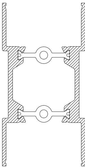
CS457 WINDOW MIDRAIL
