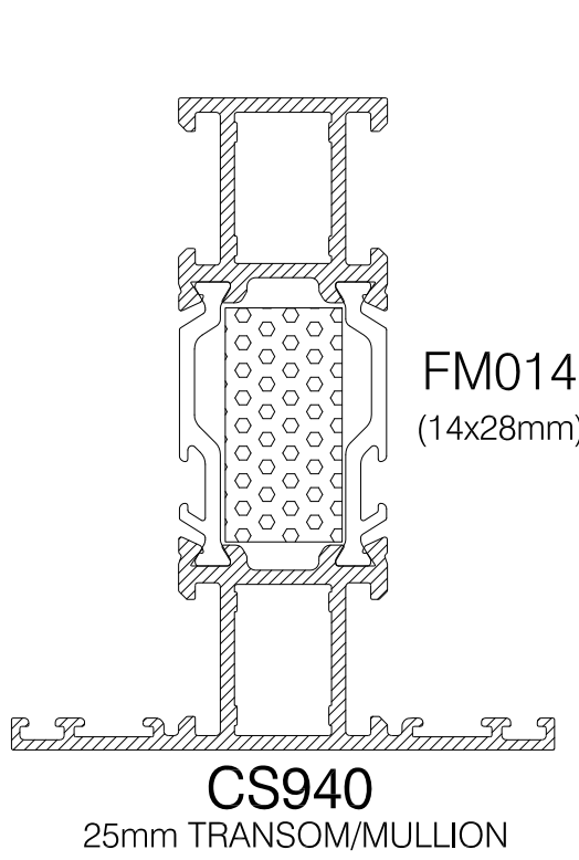
CS940 25mm TRANSOM/MULLION
