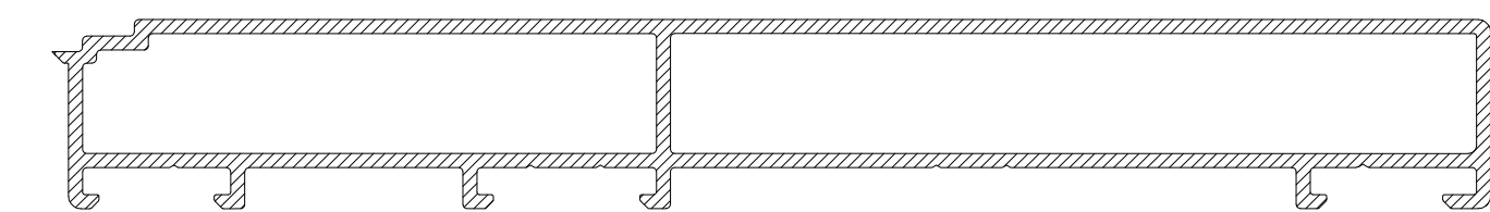
CS7510 TRIPLE TRACK JAMB (FIXED LIGHT)
