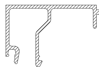
10-964 GLAZING BEAD 40mm
