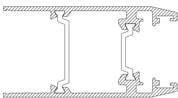
CS460 LEAF STILE
