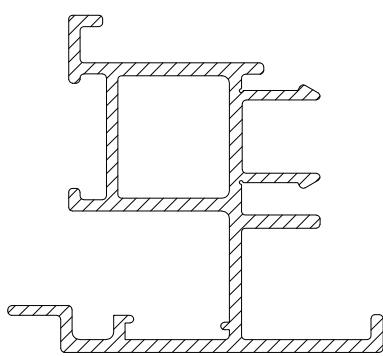
AT225 DOUBLE DOOR ADAPTER OPEN OUT
