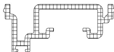
GK7010 KEEP CARRIER
