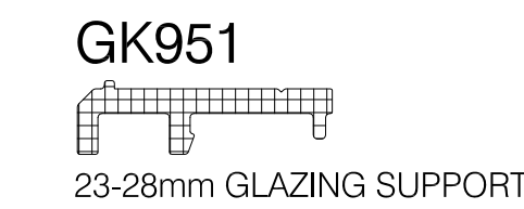
GK951 23-28mm GLAZING SUPPORT
