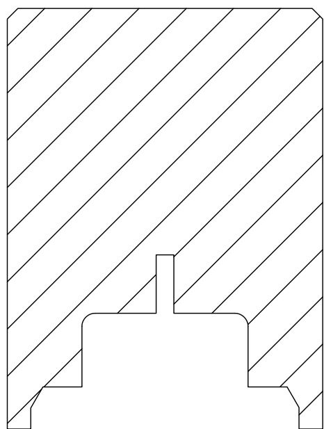
AT601 MULLION 80mm
