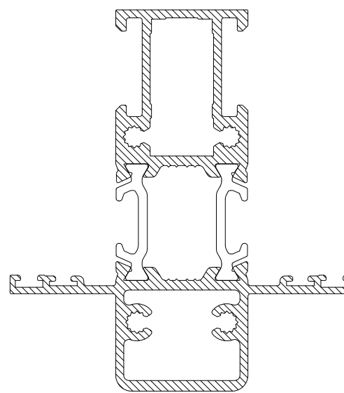
CS865 HIGH SPAN MULLION
