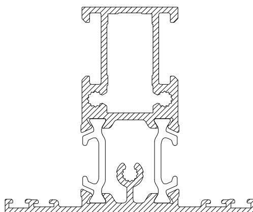
CS867 MEETING STILE ECO DOOR MULLION
