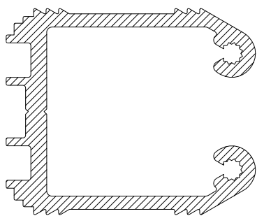
CS735 DOOR SASH SCREW TIE - ROD CLEAT AVAILABLE IN BAR LENGTH ONLY
