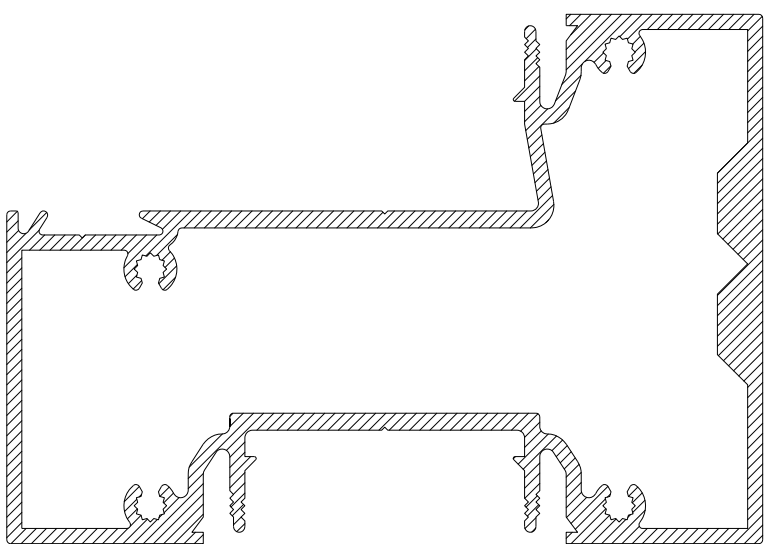
CS312 70mm AUTO BEAM TRANSOM
