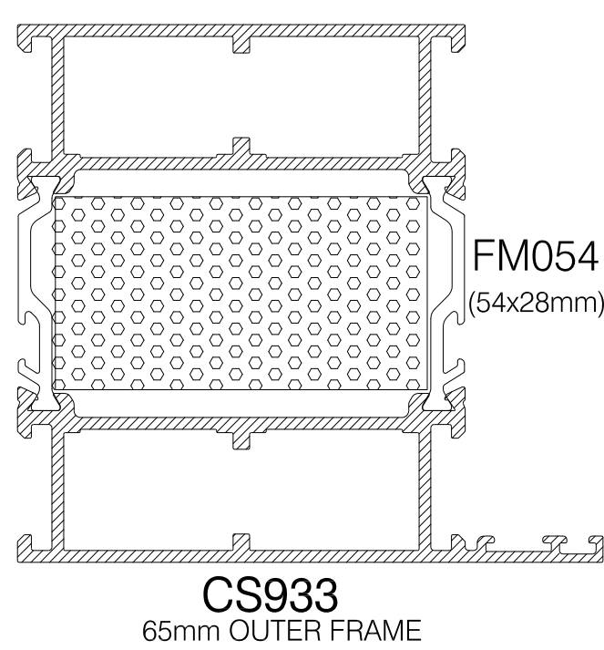
CS933 65mm OUTER FRAME
