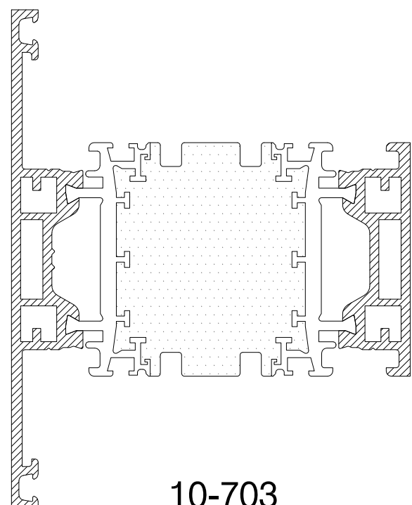
10-703 75mm TRANSOM / MULLION
