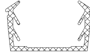
GK428 27 - 29mm GLASS GLAZING GASKET
