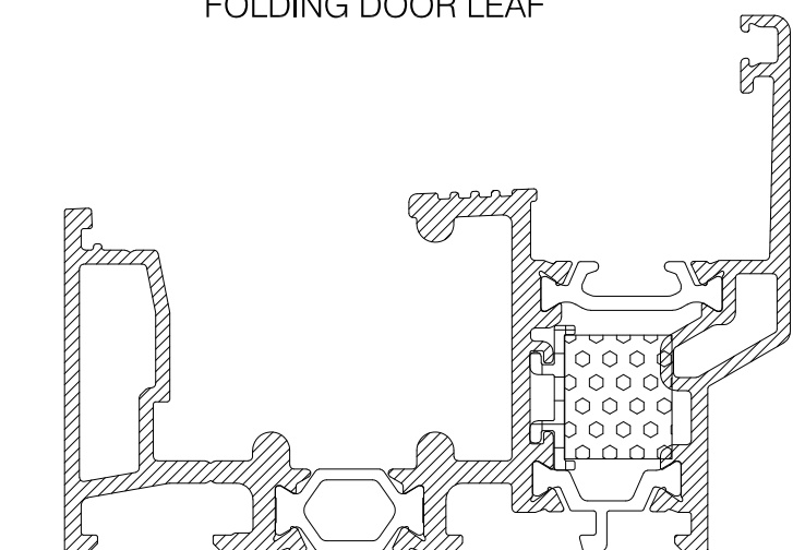
CS7003 HEAD & SILL TRACK REBATED
