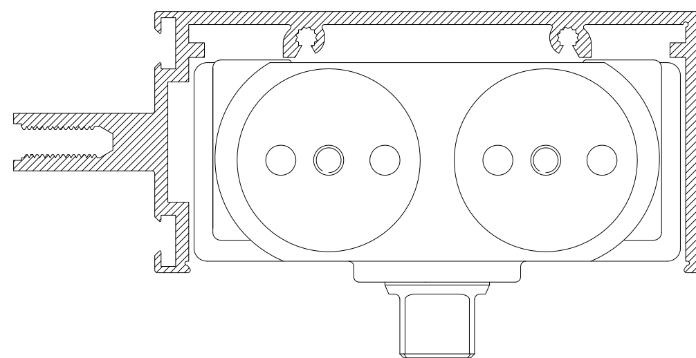
CS658 104mm LADDER FRAME HEADER BAR
