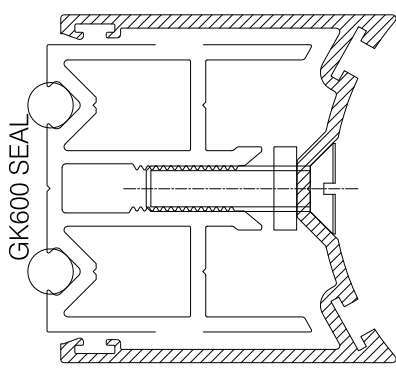
CS790 ADJUSTABLE FINGER GUARD
