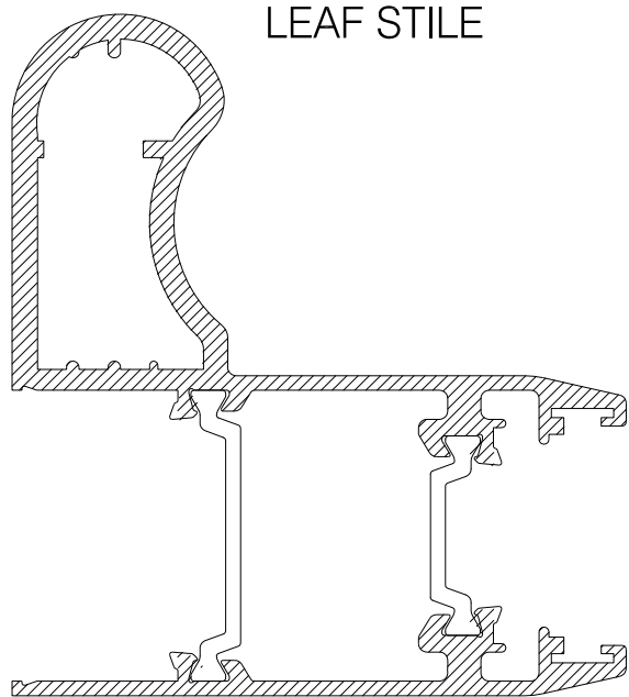
CS470 LEAF STILE WITH SINGLE HANDLE
