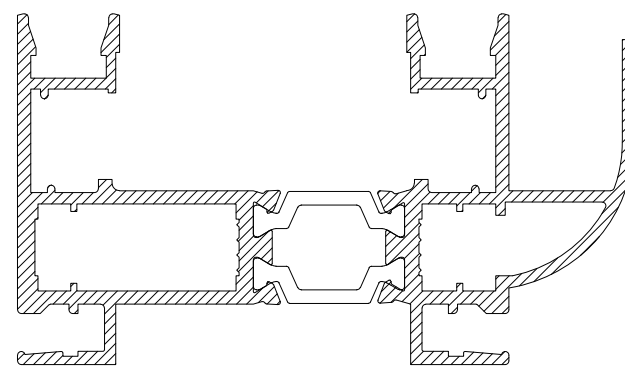
CS464 FEATURE WINDOW OUTER FRAME
