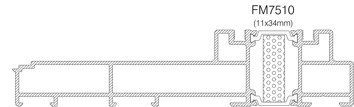
CS7509 TRIPLE TRACK JAMB (SLIDING LEAF)
