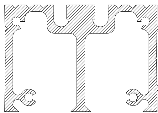
CS057 45mm SLIDING DOOR TRACK
