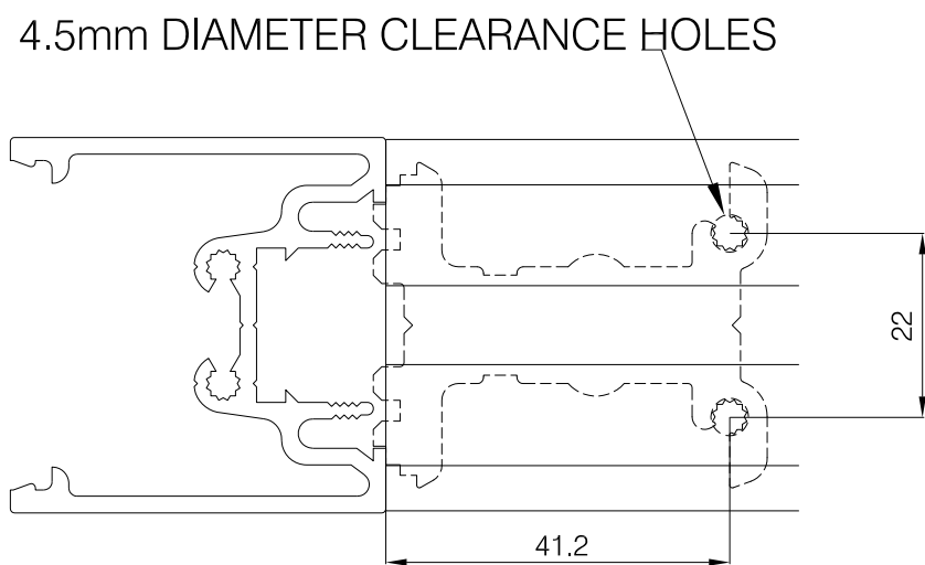
SCREW LOCATION RAIL PREPARATION FOR CS034, CS035 AND CS735
