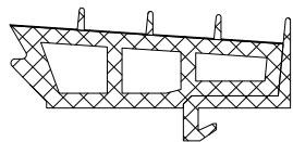
GK015 CENTRE INSULATION GASKET
