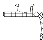
GK7017 CONTINUOUS HEAD & SILL COED FLIPPER
