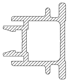
CS542 MEETING STILE LOCKING INSERT
