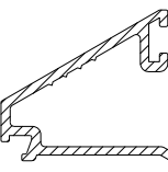
CS826 GLAZING BEAD FOR 24 MM GLASS
