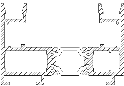
CS462 WINDOW OUTER FRAME
