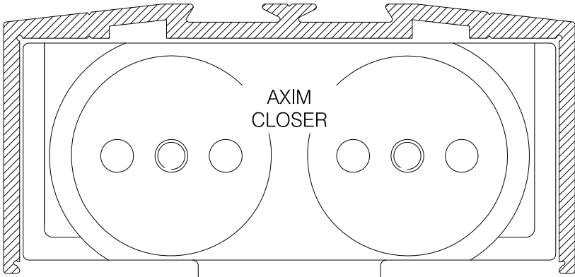
CS163 COMAR 1 OR COMAR 3 HEADER BAR WITH GLAZING ABOVE
