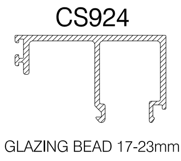
CS924 GLAZING BEAD 17-23mm
