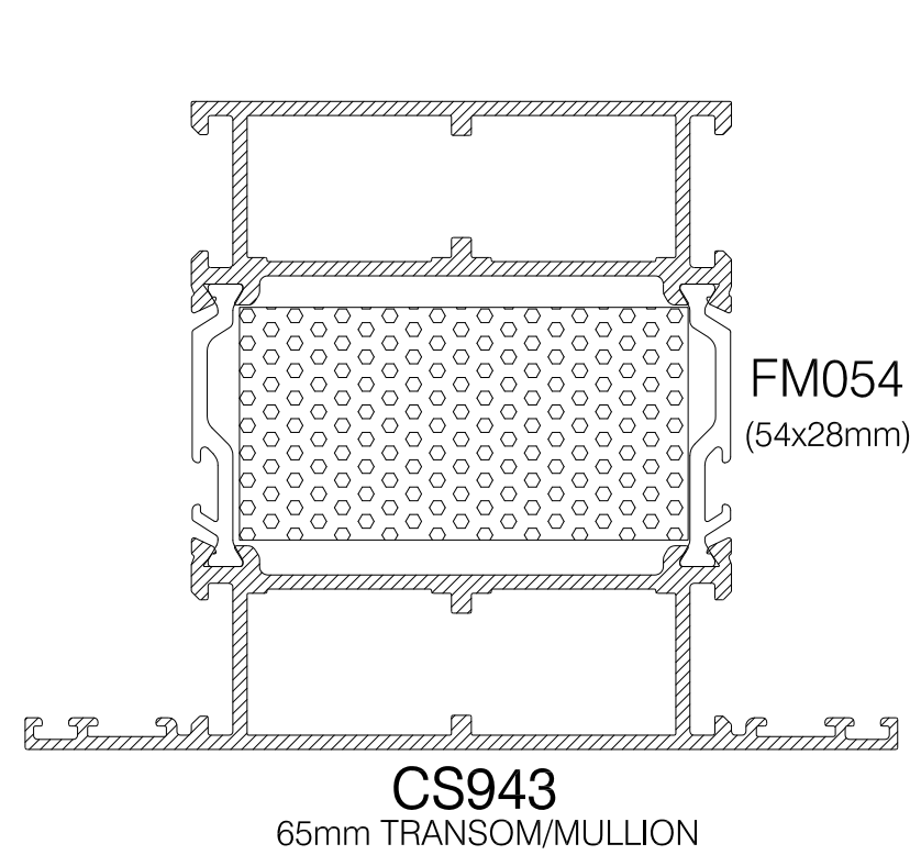
CS943 65mm TRANSOM/MULLION
