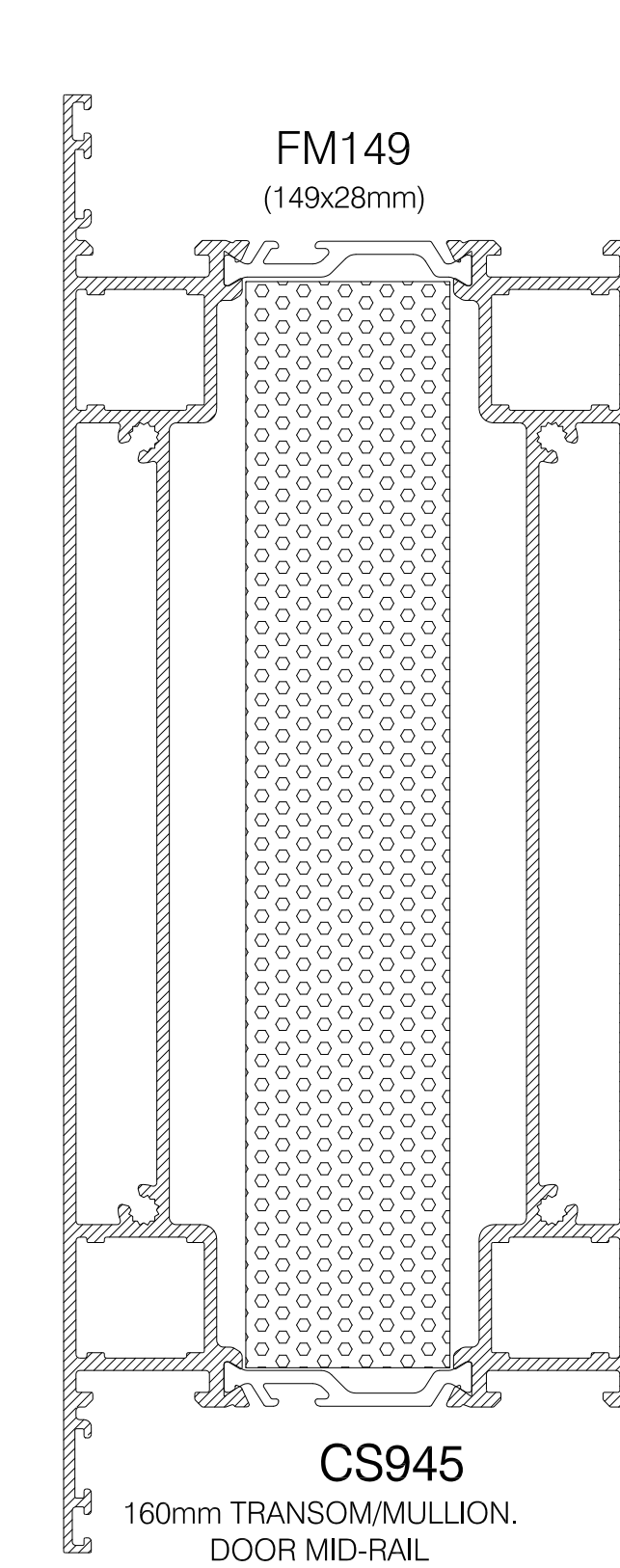
CS945 160mm TRANSOM/MULLION. DOOR MID-RAIL
