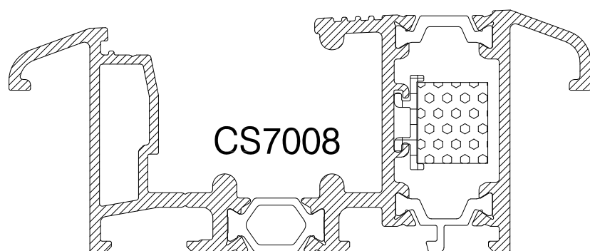
DOUBLE RAMP SILL TRACK
