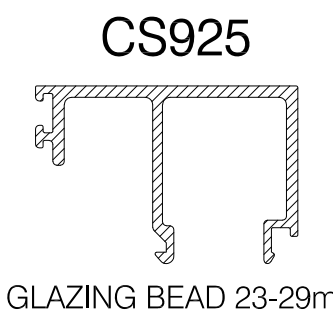
GLAZING BEAD 23-29mm
