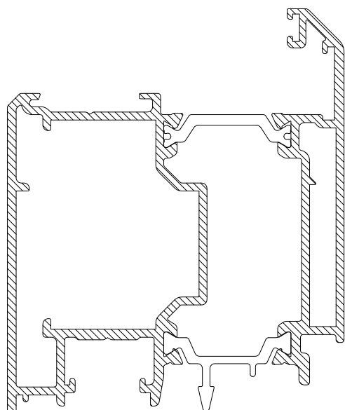
CS863 ECO DOOR LEAF OPEN IN
