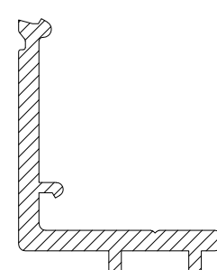
CS797 SECURITY BEAD INTERNAL
