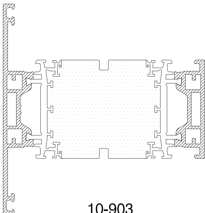
10-903 90mm TRANSOM / MULLION
