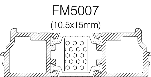
CS7506 LOCKING INSERT
