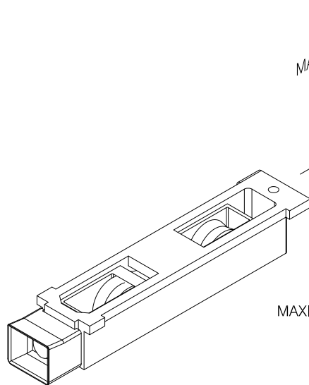
AC018XSLF WHEEL SET
