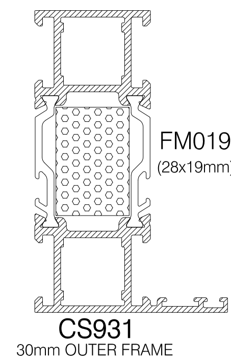
CS931 30mm OUTER FRAME
