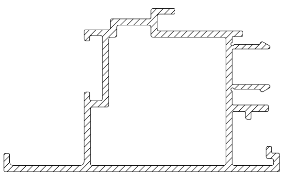
AT224 DOUBLE DOOR ADAPTER OPEN IN
