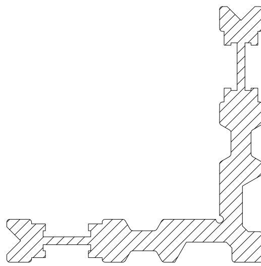
CS246 11mm WINDOW CLEAT
