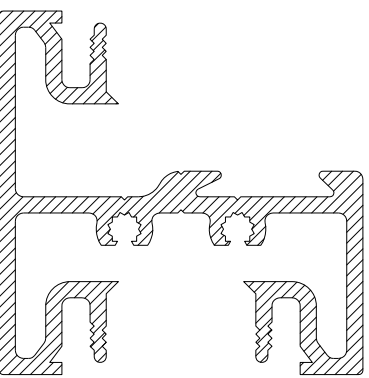
CS111 45mm TRANSOM MULLION
