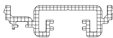
GK7009 MULTI POINT LOCK CARRIER
