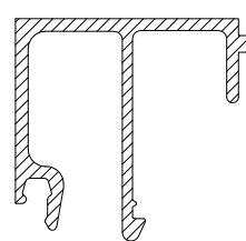
10-962 GLAZING BEAD 28mm
