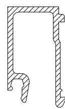
10-953 GLAZING BEAD 15mm
