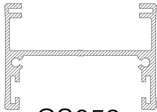
CS059 45mm SLIDING DOOR FRAME HEAD OR JAMB
