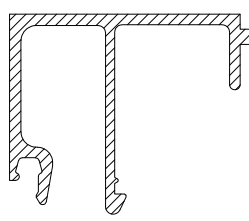
10-957 GLAZING BEAD 32mm
