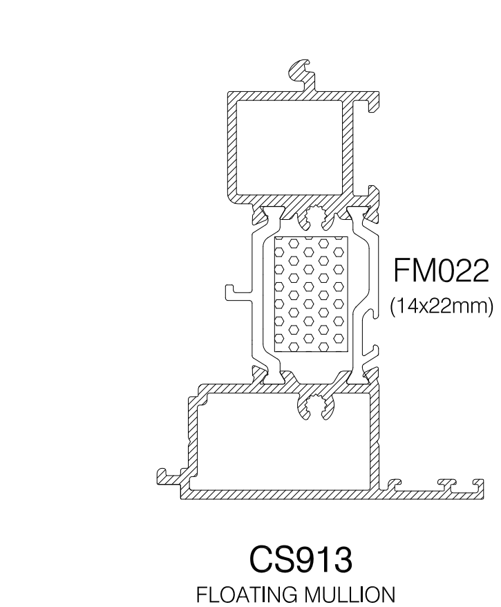
CS913 FLOATING MULLION
