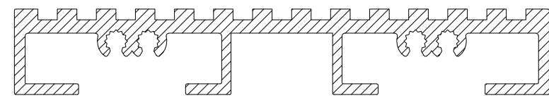
CS715 SQUARE RAMP THRESHOLD
