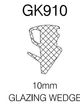
GK910 10mm GLAZING WEDGE
