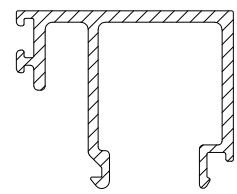
CS926 GLAZING BEAD
