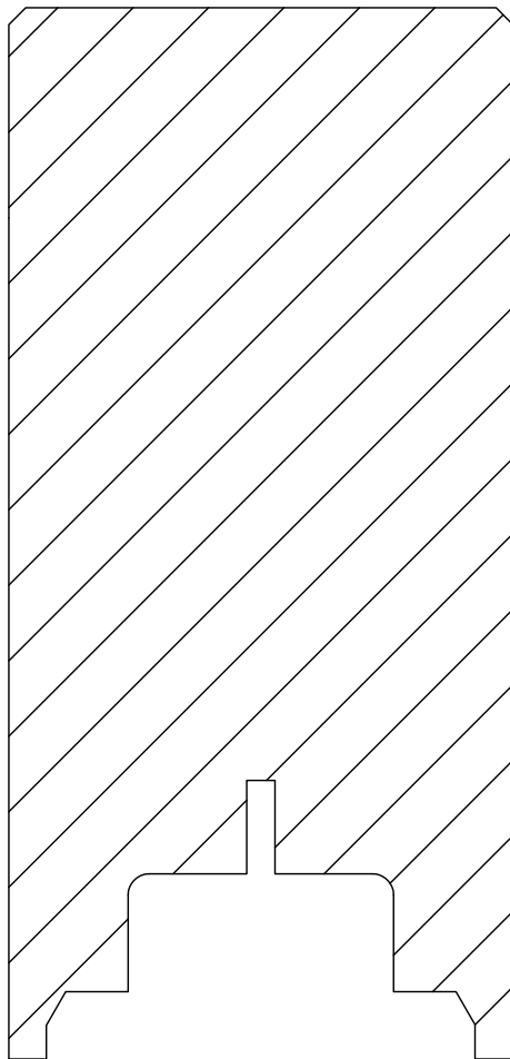
AT605 MULLION 125mm
