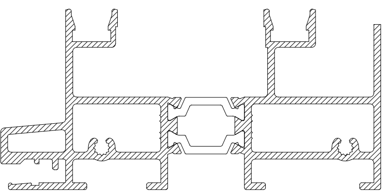
CS474 2 TRACK SLIDING DOOR OUTER FRAME SILL
