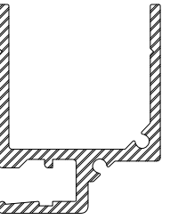
CS685 SUB SILL CARRIER
