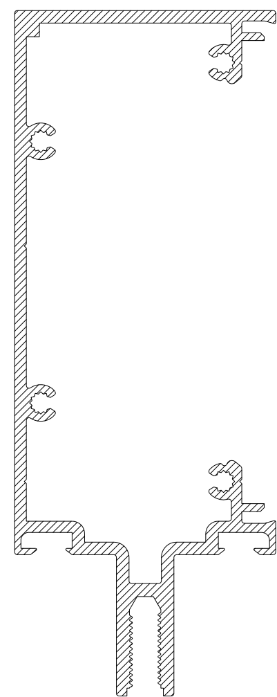
CS666 INFILL PLATE
