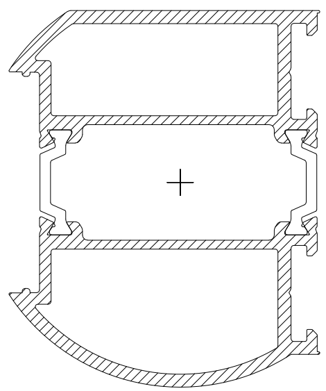
CS774 FINGER GUARD DOOR STILE, PANIC EXIT
