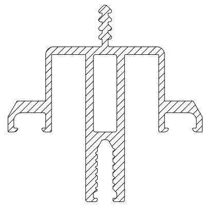
AT1065 MULLION
