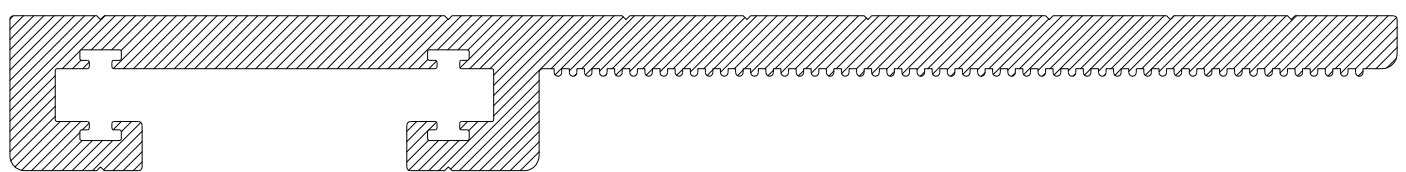
CS904 JAMB BRACKET COMPONENT
