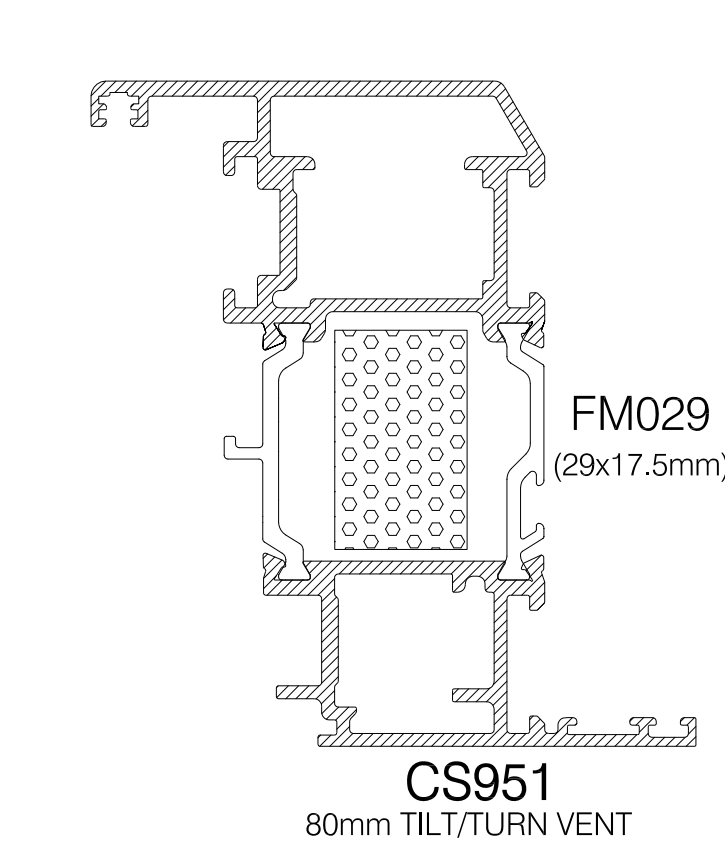
CS951 80mm TILT/TURN VENT
