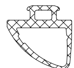
GK7005 BI-PART COMPRESSION SEAL 'A'
