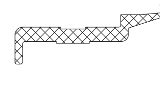
GK546 OVERLAP STILE INTERLOCK INSERT
