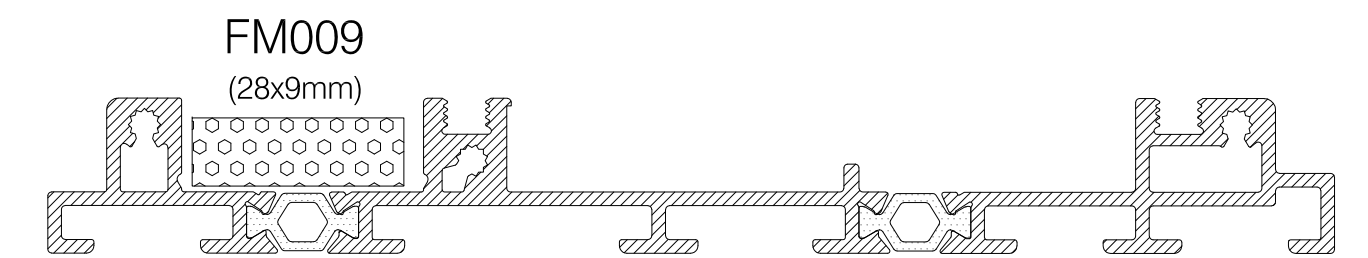
CS7503 DOUBLE TRACK LOW THRESHOLD
