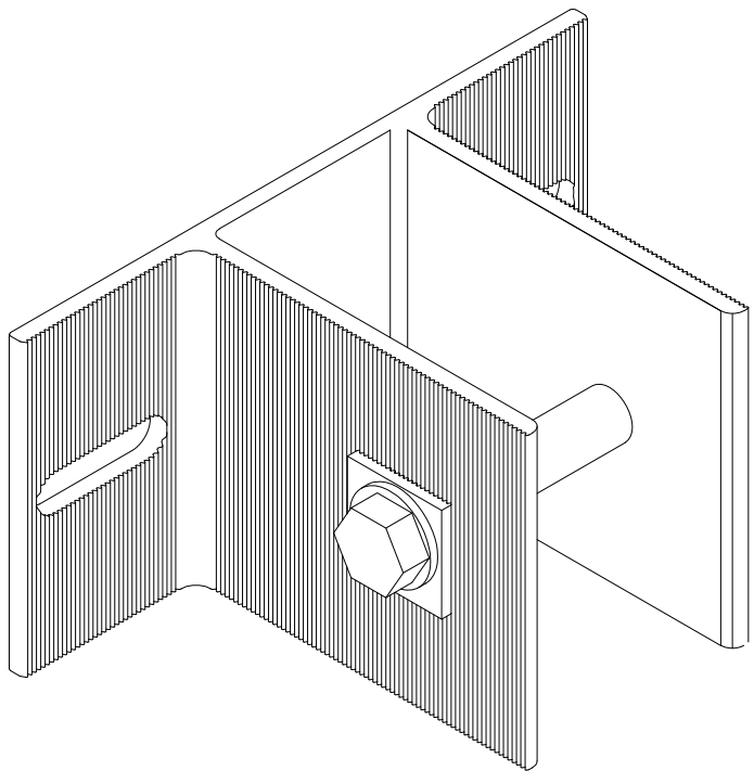
XX6092XKIT Bracket Fixed 60mm Kit
