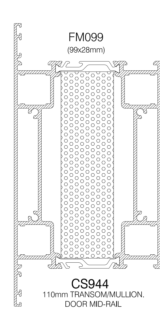
CS944 110mm TRANSOM/MULLION. DOOR MID-RAIL
