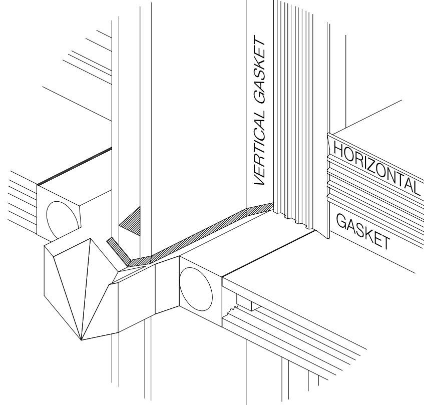
CW051XSLF 27.2mm DRAINAGE SPOUT FOR USE WITH GK619 ISOLATOR
