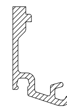
10-958 GLAZING BEAD 5mm
