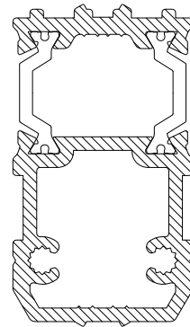
CS843 45mm COUPLER
