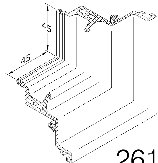
2613 EFT 4003 WINDOW AIR SEAL MOULDED CORNER 45X45mm
