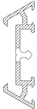
CS674 14.5mm PRESSURE PLATE / COVER CAP PRE PUNCHED
