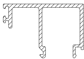
CS925 GLAZING BEAD
