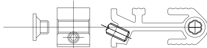
WS918XKIT 14.5mm CLEAT (FOR CS7522) 1 x M5x10mm GRUB SCREW 1 x M6x7mm CSK SCREW
