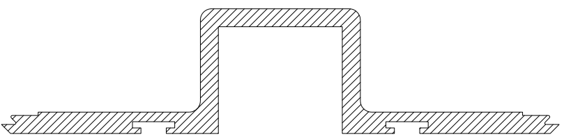
CS042 SLIDING FOLDING DOOR'S HEADER BAR
