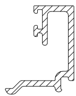
CS929 GLAZING BEAD
