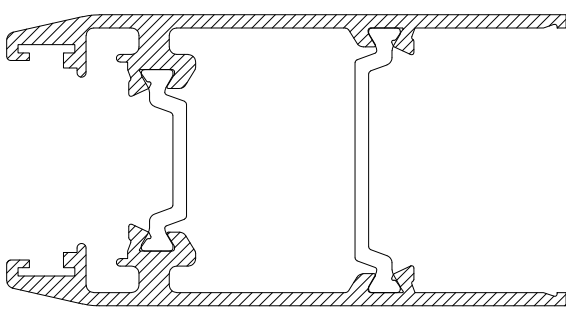
CS460 WINDOW STILE
