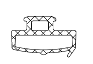
JAMB COMPRESSION SEAL
