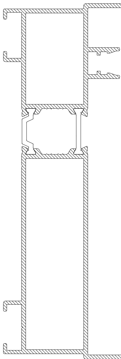
CS478 3 TRACK SLIDING DOOR OUTER FRAME JAMB
