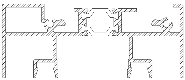
CS468 2 TRACK SLIDING DOOR OUTER FRAME HEAD
