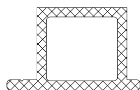
GK628 CURTAIN WALL WINDOW INSERT
