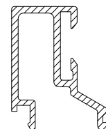
CS227 DOUBLE GLAZING WINDOW BEAD (SQUARE)
