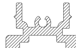
CS786 8mm SIDE WING CARRIER
