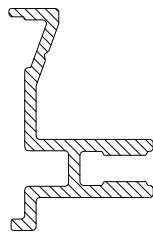
CS858 OPEN OUT DOOR REBATE ADAPTER
