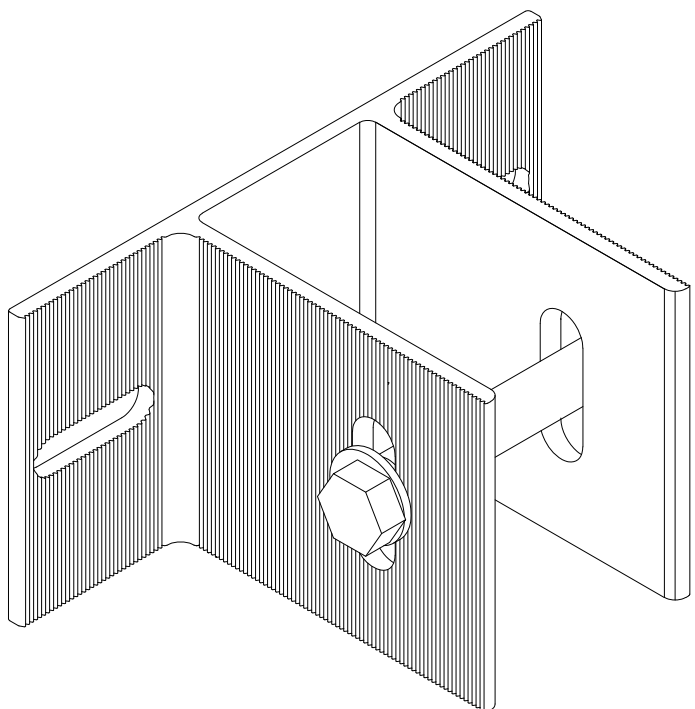
XX6093XKIT Bracket Sliding 60mm Kit
