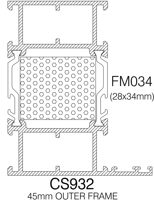
CS932 45mm OUTER FRAME
