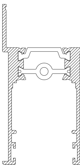
CS461 LEAF BOTTOM OR TOP RAIL
