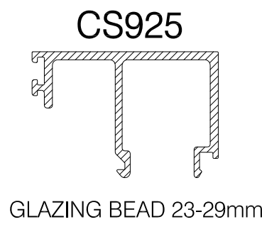
CS925 GLAZING BEAD 23-29mm
