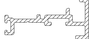
CS914 LOW THRESHOLD GASKET CARRIER OPEN IN
