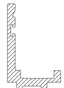
CS796 SECURITY BEAD EXTERNAL
