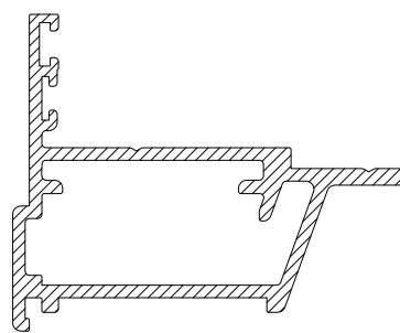
CS864 TRANSFER PROFILE
