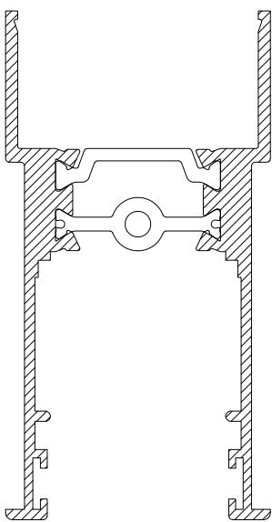
CS461 WINDOW TOP OR BOTTOM RAIL
