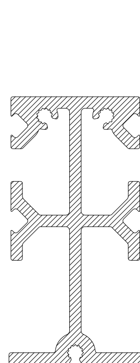
CS656 CURTAIN WALL 70mm SPIGOT
