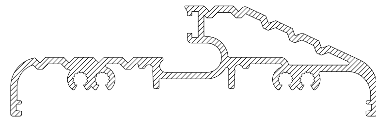
CS347 HINGED REBATED DOOR DRAINED THRESHOLD
