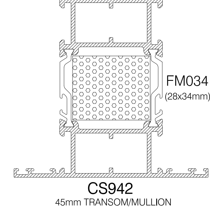
CS942 45mm TRANSOM/MULLION
