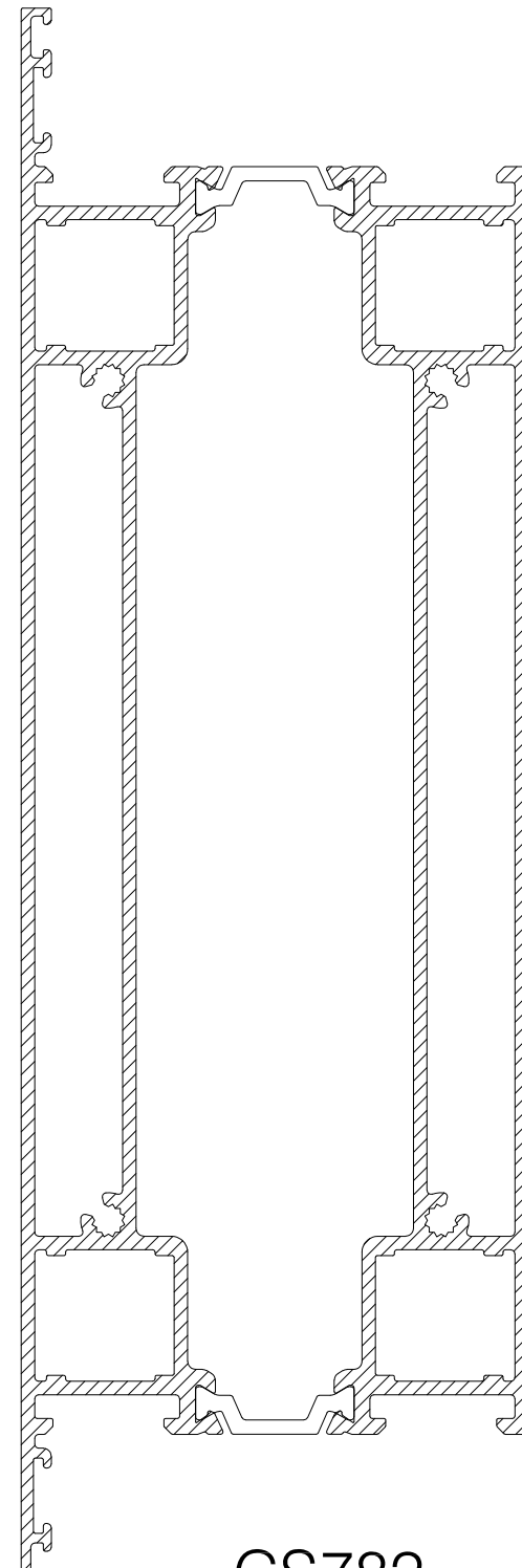
CS782 200mm TRANSOM/MIDRAIL
