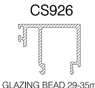
GLAZING BEAD 29-35mm
