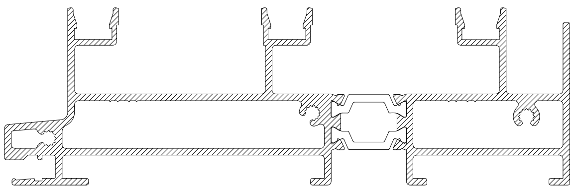
CS479 3 TRACK SLIDING DOOR OUTER FRAME SILL
