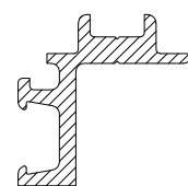
10-911 CURTAIN WALL ADAPTOR
