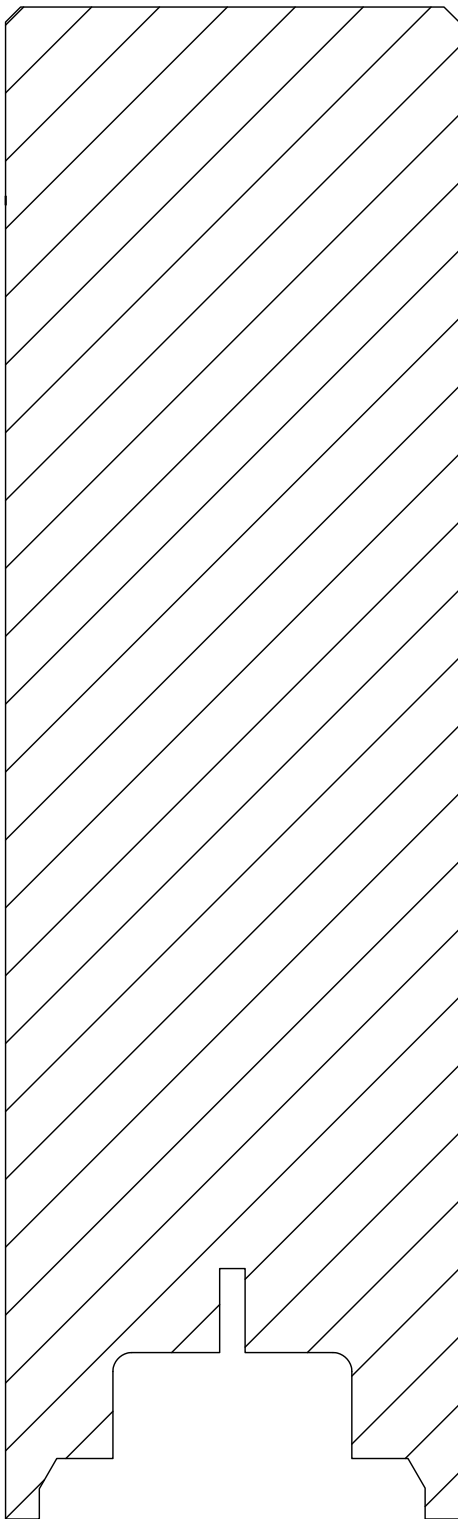
AT607 MULLION 200mm
