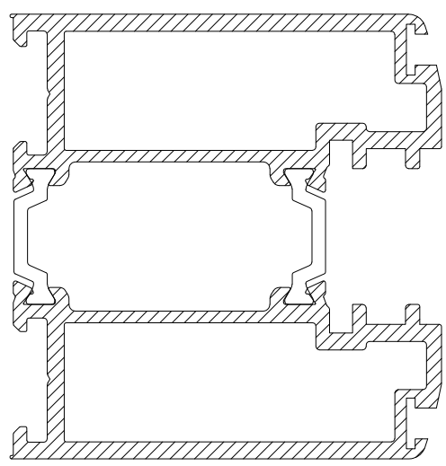
CS779 DOOR STILE WOOLPILE
