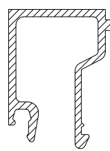
10-960 GLAZING BEAD 20mm
