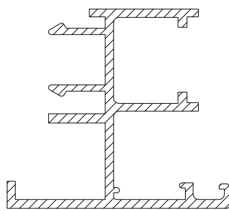
AT221 VENT FRAME ADAPTER
