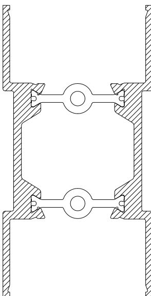
CS457 LEAF MIDRAIL
