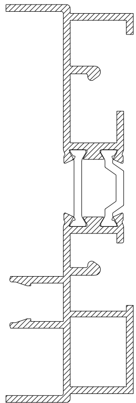
CS466 2 TRACK DOOR OUTSIDE TRACK JAMB
