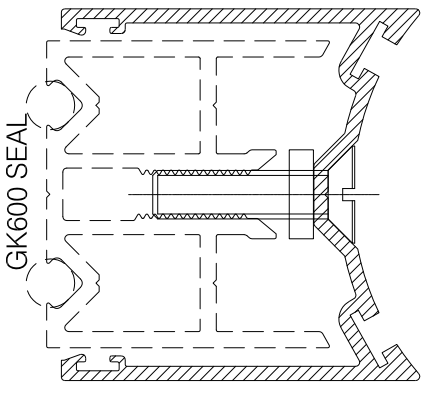
CS790 ADJUSTABLE FINGER GUARD
