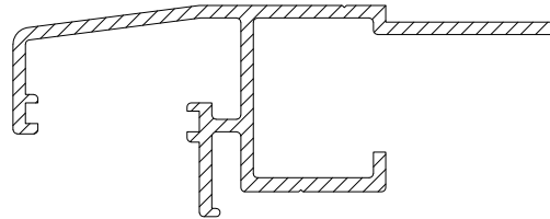
AT204 NIGHT VENT HOOD ALUMINIUM
