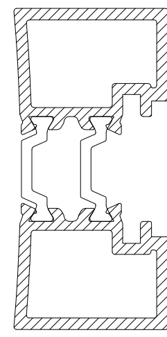
CS997 MULLION ADAPTOR
