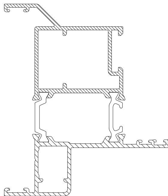
CS5816 85mm DOOR OUTER FRAME
