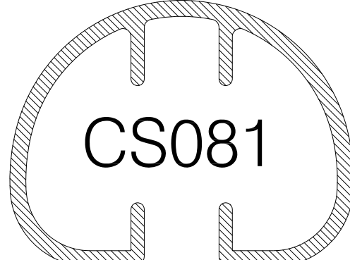
CS081 ARMOURED GLASS FINGER GUARD STILE
