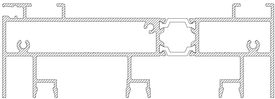
CS477 3 TRACK SLIDING DOOR OUTER FRAME HEAD
