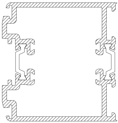
CS771 DOOR STILE (T.B) (T.B) = THERMALLY BROKEN PROFILE
