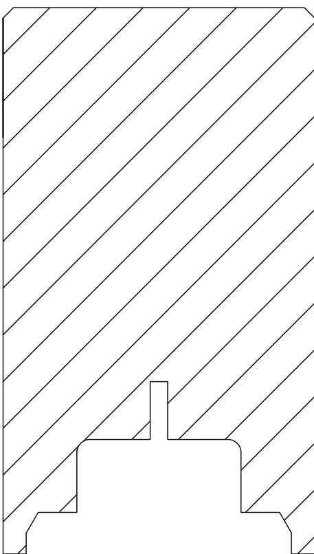
AT602 MULLION 105mm
