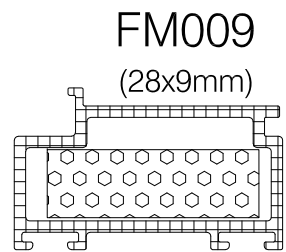
FM009 (28x9mm) LEAF INSULATION BOX
