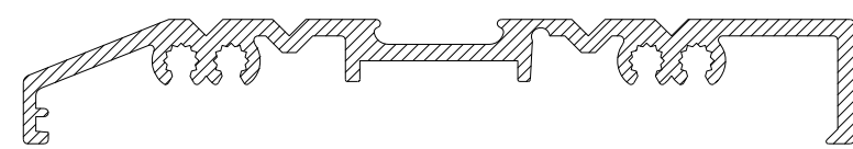
CS345 SINGLE RAMP DRAINED THRESHOLD
