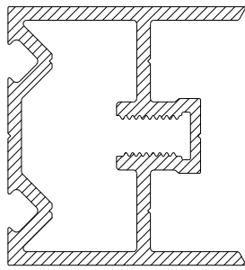
CS791 ADJUSTABLE FINGER GUARD FIXING CHANNEL
