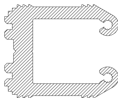
CS035 DOOR SASH SCREW CLEAT AVAILABLE IN BAR LENGTH OR CUT SIZES
