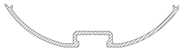
CS874 ECO BAY POLE 150° COVER CAP
