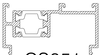
CS851 ECO 55 FRAME EXTENSION
