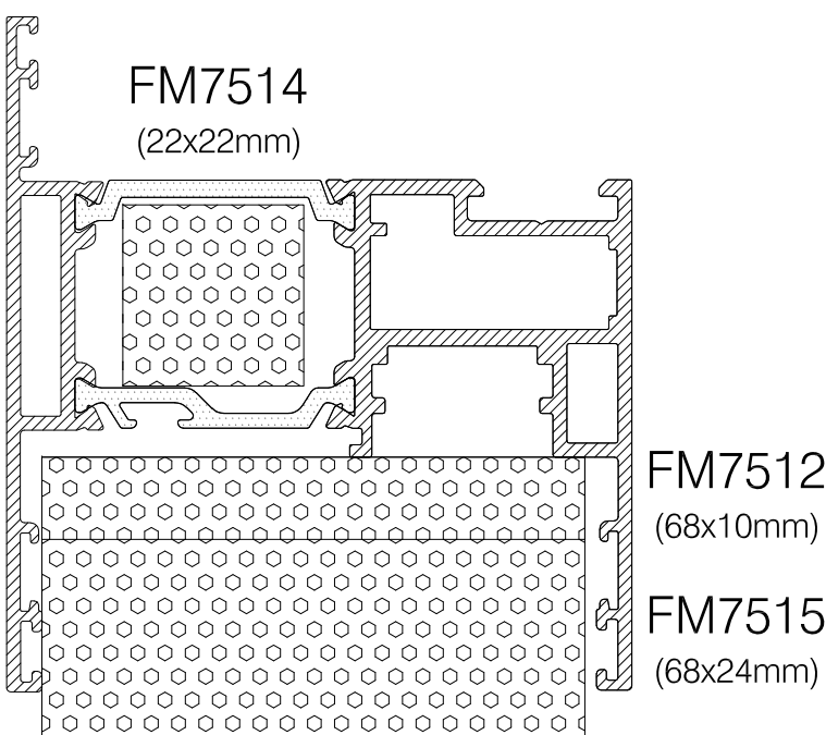
CS7517 STANDARD LEAF
