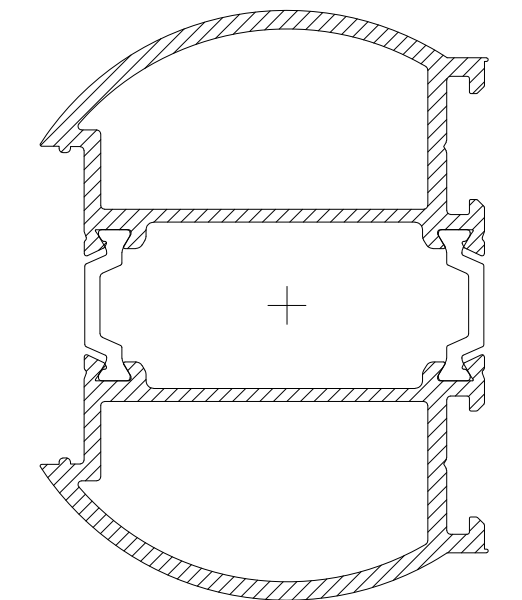
CS773 FINGER GUARD DOOR STILE
