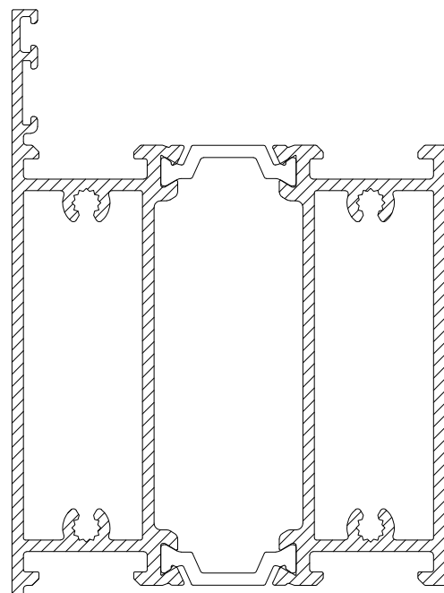
CS780 105mm TRANSOM/MIDRAIL
