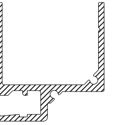
CS686 SUB SILL CARRIER
