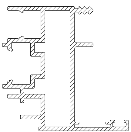
AT211 VENT FRAME ALUMINIUM
