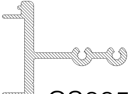
CS335 DOUBLE GLAZED 63mm SASH RAIL CLEAT
