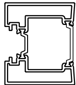
CS998 52mm Mullion Adapter
