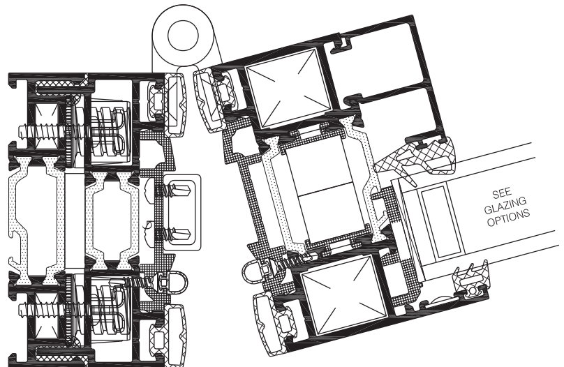
General Arrangement showing Comar 7P.i FSD, folding/sliding in
