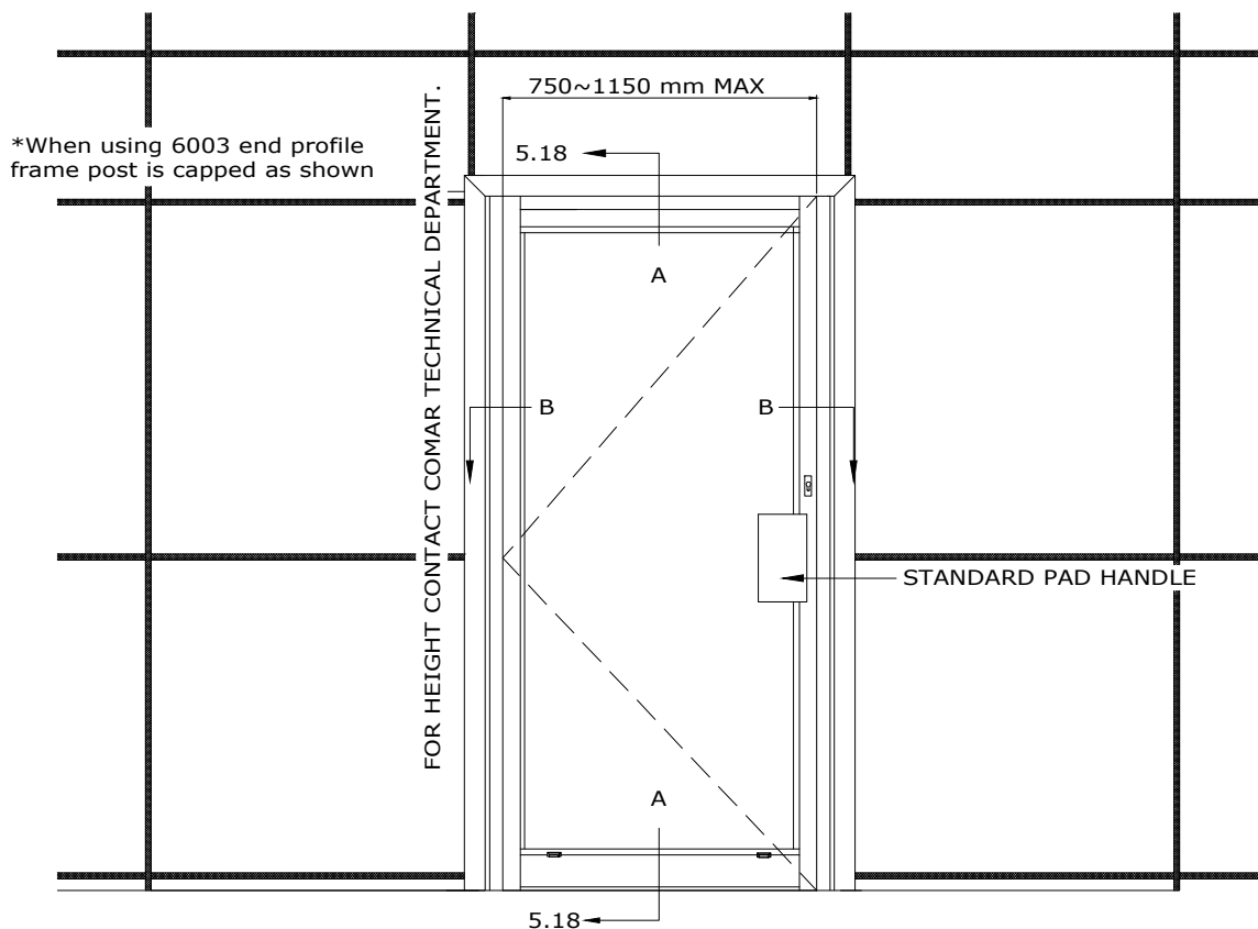
EXTERNAL ELEVATION (COMAR 7 STANDARD SWING DOOR)
