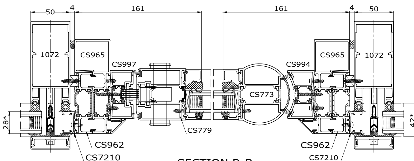
SECTION B-B
