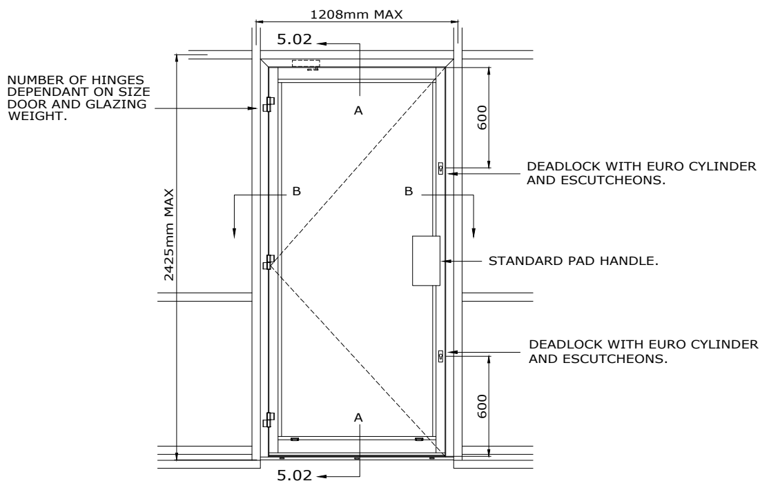
EXTERNAL ELEVATION (COMAR 7 REBATED DOOR)
