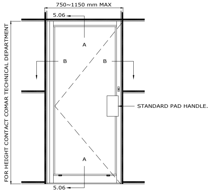
EXTERNAL ELEVATION (COMAR 7 ANTI FINGER TRAP DOOR)
