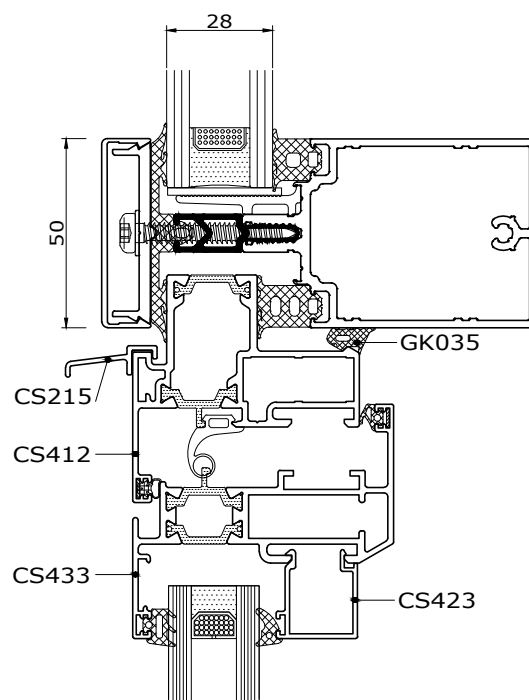
TILT TURN / BOTTOM HUNG, OPEN IN. 5Pi 60mm WINDOW SYSTEM INTERNALLY BEADED
