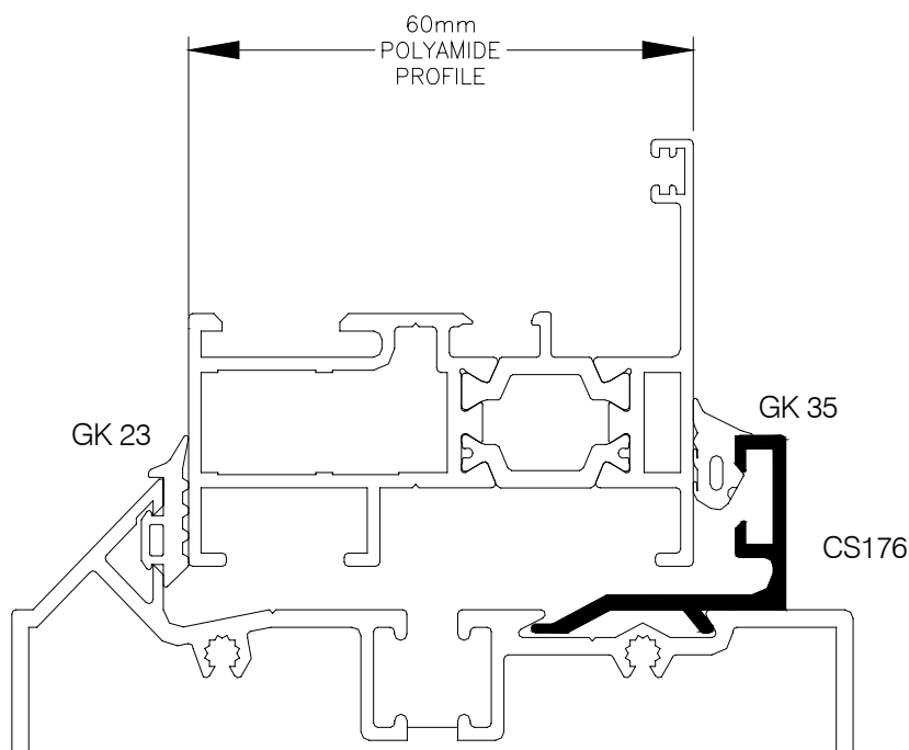
STD. COMAR 2 MULLION/ TRANSOM SECTION. (20mm HIGH INTERNAL GLAZING BEAD.)
