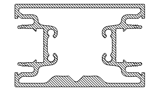
CS103 CILL/TRANSOM AUTO BEAM
