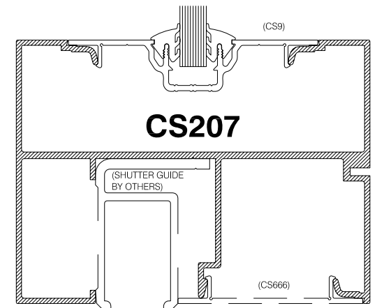
CS206 100mm x 100mm FRAME MULLION
