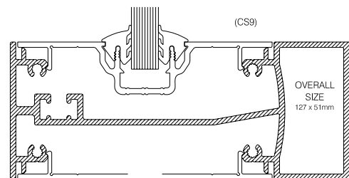
CS148 HIGH SPAN MULLION (NOT THERMALLY BROKEN)
