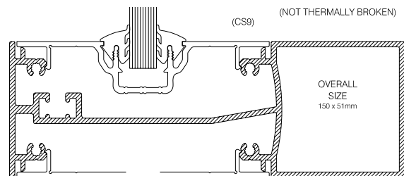
CS178 HIGH SPAN MULLION (NOT THERMALLY BROKEN)
