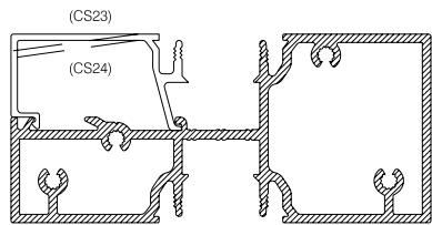
CS5 SILL/TRANSOM (BOX) (AMENDED PORTS)
