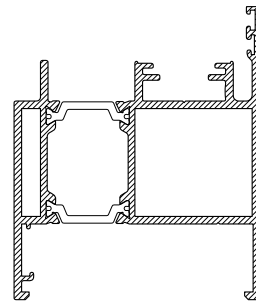
CS768 OUTWARD OPENING DOOR LONG LEGGED OUTER FRAME
