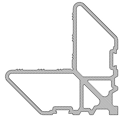
42.5mm CLEAT CS792
