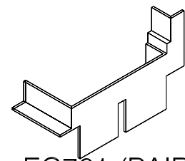
EC761 (PAIR) DOUBLE DOOR STOP FLASHING PIECE HANDED
