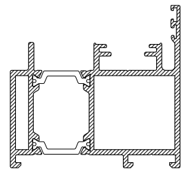
CS760 OUTWARD OPENING DOOR OUTER FRAME
