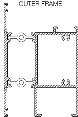
CS764 SQUARE CUT BOTTOM RAIL
