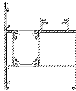
CS769 INWARD OPENING DOOR LONG LEGGED OUTER FRAME
