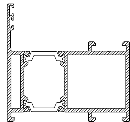
CS765 OUTER FRAME
