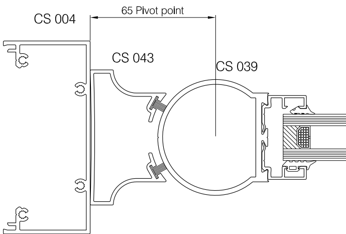
COMAR 1 & 3 FRAMEWORK
