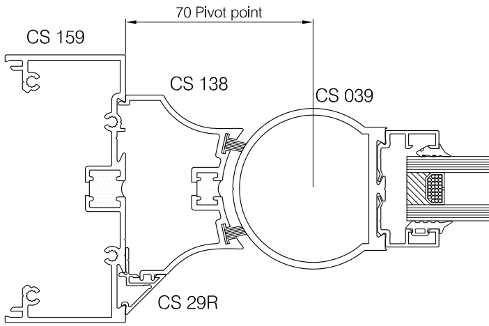
COMAR 2 FRAMEWORK
