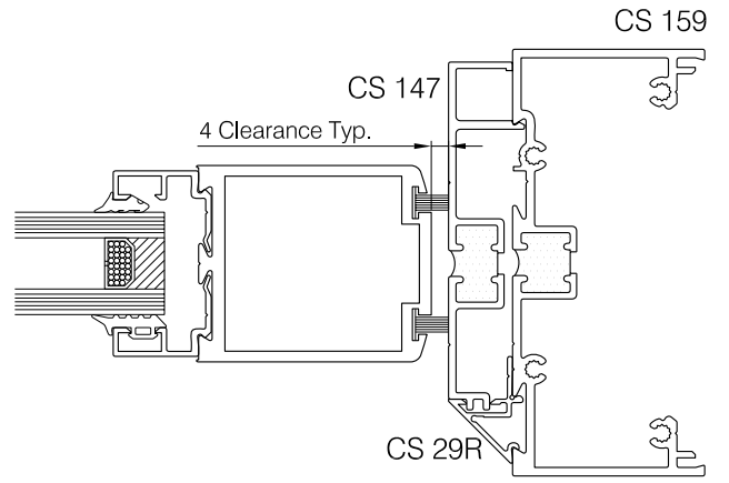
COMAR 2 FRAMEWORK
