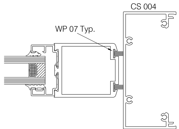
COMAR 1 & 3 FRAMEWORK
