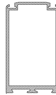
CS56R 80mm WIDE DOOR STILE (WOOLPILE)
