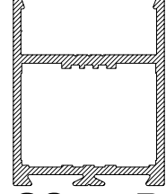
CS717R 55mm DOOR/SASH RAIL REVISED (ECONOMY)
