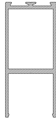
CS18 100mm DOOR/SASH RAIL
