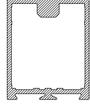
CS727R 55mm AUTOMATIC DOOR RAIL REVISED (ECONOMY)
