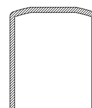
CS70 80mm WIDE DOOR STILE (PLAIN)
