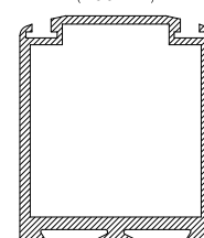
CS16R 55mm DOOR STILE (WOOLPILE)
