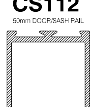
CS112 50mm DOOR/SASH RAIL
