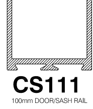
CS111 100mm DOOR/SASH RAIL
