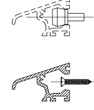
CS83 SCREW OR CLIP FIT DRIP SECTION FX046SLF STUD & FX045SLF FIXING, FX047SLF PROFILE RIVET
