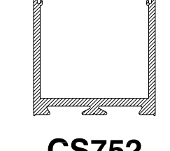
CS752 55mm DOOR STILE OPEN BACK (PLAIN)
