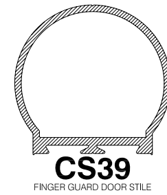
CS39 FINGER GUARD DOOR STILE
