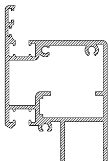
CS714 TEMPEST 2000 REBATED DOOR FRAME (COMAR 6)
