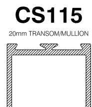
CS115 20mm TRANSOM/MULLION
