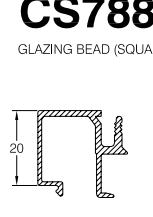
CS373 GLAZING BEAD (DOUBLE GLAZE)
