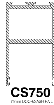
CS750 75mm DOOR/SASH RAIL
