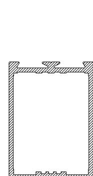
CS718R 100mm DOOR/SASH RAIL REVISED (ECONOMY)
