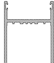
CS740R 75mm DOOR/SASH RAIL REVISED (ECONOMY)
