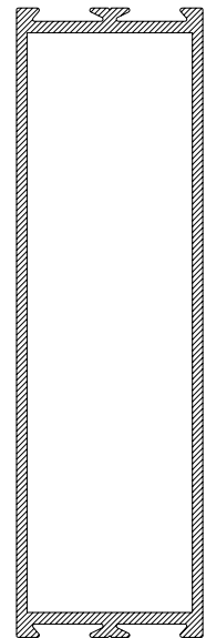
CS38 150mm DOOR/SASH RAIL
