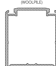
CS716R 55mm DOOR STILE WOOLPILE (ECONOMY)
