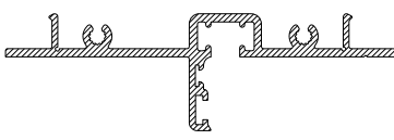
CS712 TEMPEST 2000 REBATED DOOR FRAME (COMAR 2)
