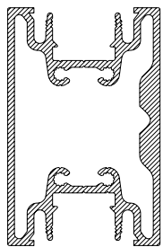
CS103 175 x 45 CILL / TRANSOM AUTO BEAM
