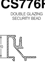
CS776R DOUBLE GLAZING SECURITY BEAD
