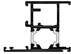
CS441 SLIDING WINDOW LOWER SASH
