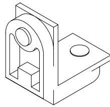
WS389XSLF CORNER CLEAT MC0389 FOR CS456
