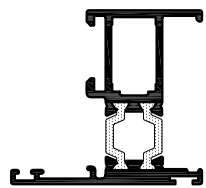
CS443 SLIDING WINDOW UPPER SASH
