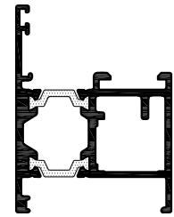
CS442 SLIDING WINDOW LOWER SASH
