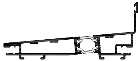
CS450 SLIDING WINDOW SILL
