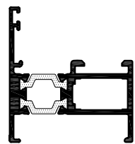
CS444 SLIDING WINDOW UPPER SASH
