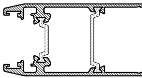
CS460 HORIZONTAL SLIDING STILE
