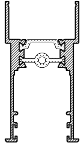
CS461 HORIZONTAL SLIDING RAIL
