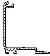
CS452 HORIZONTAL SLIDER INTERLOCK
