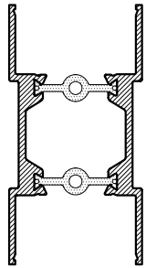
CS457 SLIDING WINDOW MIDRAIL
