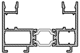
CS462 STANDARD SLIDING WINDOW FRAME
