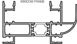
CS464 FEATURE SLIDING WINDOW FRAME
