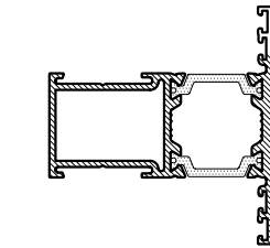
CS832 TRANSOM / MULLION
