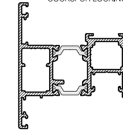
CS825 VENT (FEATURE) - EXTERNAL BEAD SHOOTBOLT LOCKING COCKSPUR LOCKING
