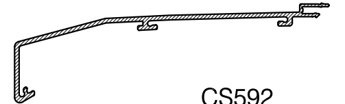
CS592 110mm SUB SILL NOSING
