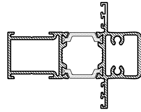
CS821 HIGH SPAN MULLION FOR OUTER FRAME CS817, CS818 (SHOOTBOLT LOCKING ONLY)
