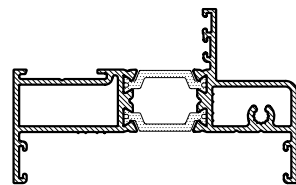
CS818 75mm FIXED LIGHT / OUTER FRAME (COCKSPUR LOCKING)
