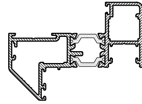
CS825 VENT (FEATURE) - EXTERNAL BEAD SHOOTBOLT LOCKING COCKSPUR LOCKING
