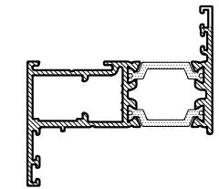
CS836 VENT (FLAT) - EXTERNAL BEAD COCKSPUR LOCKING
