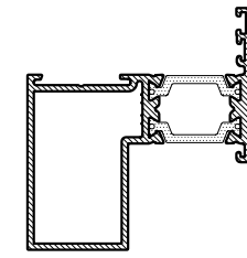
CS813 CURTAIN WALL WINDOW INSERT
