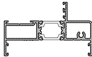
CS817 75mm FIXED LIGHT / OUTER FRAME (SHOOTBOLT LOCKING ONLY)
