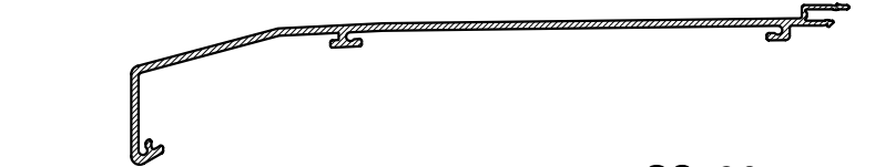
CS596 160mm SUB SILL NOSING
