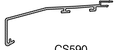
CS590 80mm SUB SILL NOSING
