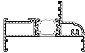
CS815 75mm FIXED LIGHT / OUTER FRAME (COCKSPUR LOCKING)
