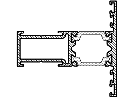
CS835 TRANSOM / MULLION
