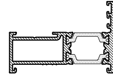
CS834 FIXED LIGHT / OUTER FRAME SHORT LEG
