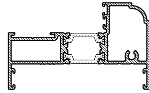
CS819 75mm FIXED LIGHT / OUTER FRAME OVOLO (SHOOTBOLT LOCKING ONLY)
