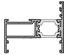
CS810 FIXED LIGHT / OUTER FRAME
