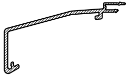
CS588 52mm SUB SILL NOSING
