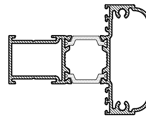
CS822 HIGH SPAN MULLION OVOLO FOR OUTER FRAME CS815, CS819 (SHOOTBOLT LOCKING ONLY)
