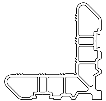
CS547 23mm WINDOW CLEAT
